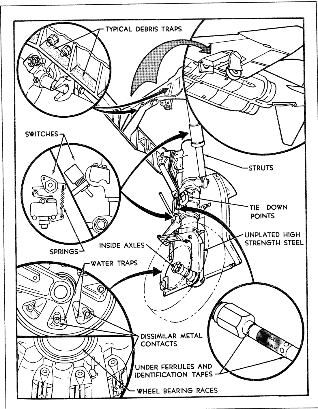
FIGURE 4-3. LANDING GEAR AND WHEEL CORROSION POINTS
