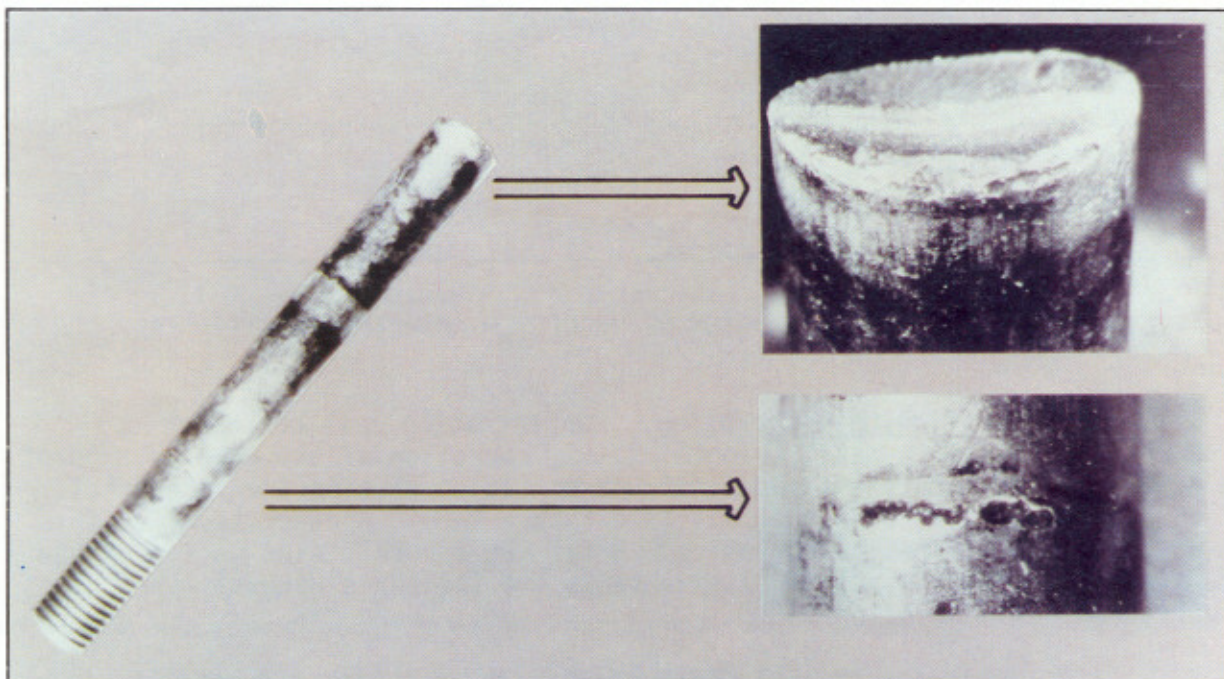
FIGURE 2-4. PITTING CORROSION
