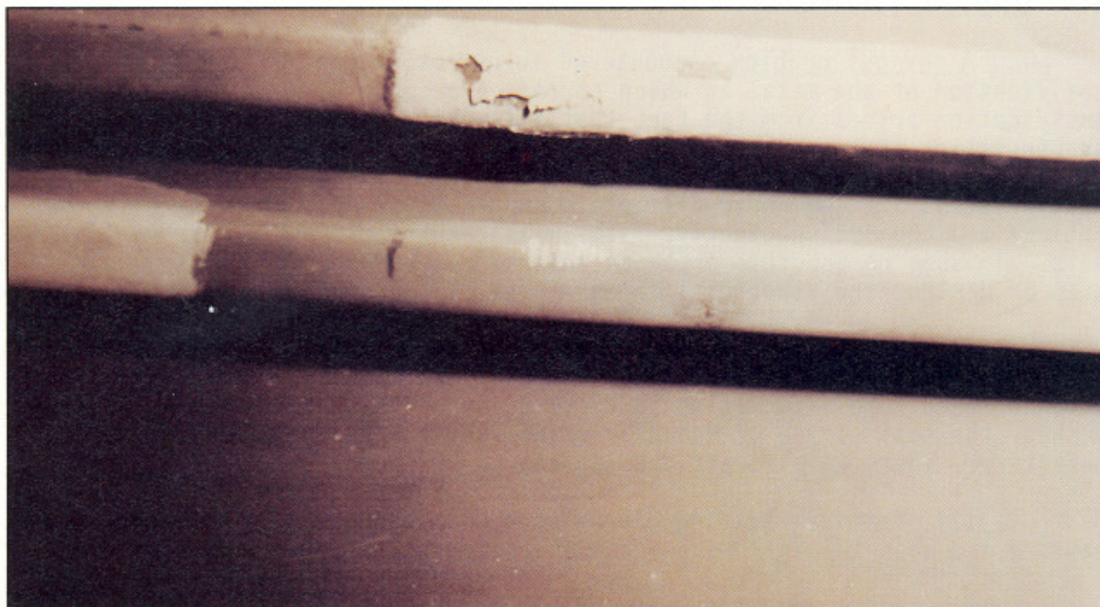
FIGURE 6-6. INCOMPLETE REMOVAL OF CORROSION PRODUCTS RESULTED IN REOCCURRENCE OF CORROSION
