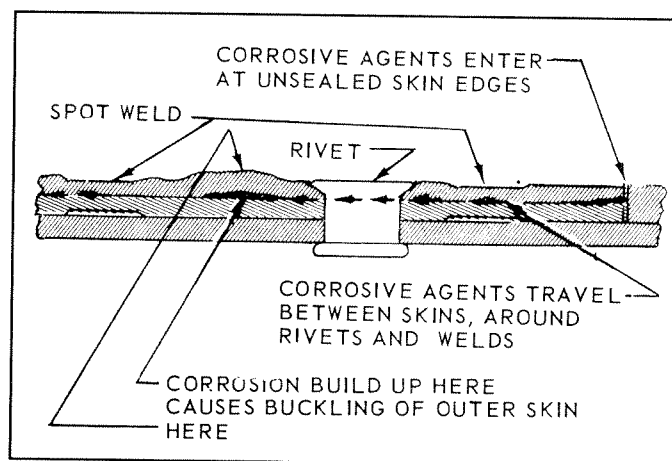
FIGURE 4-6. SPOTWELDED SKIN CORROSION
