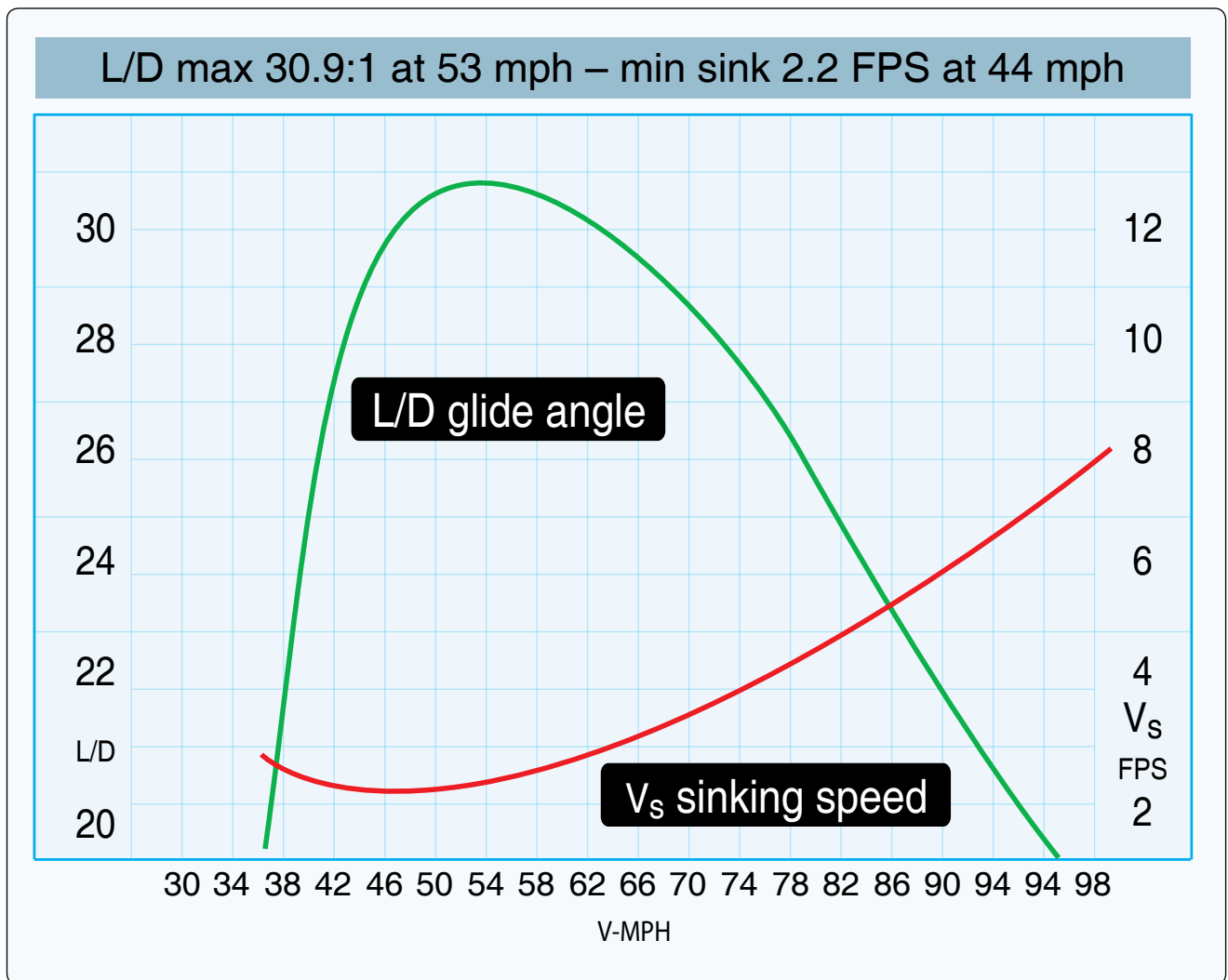
Figure 54. Glider Performance Graph.
