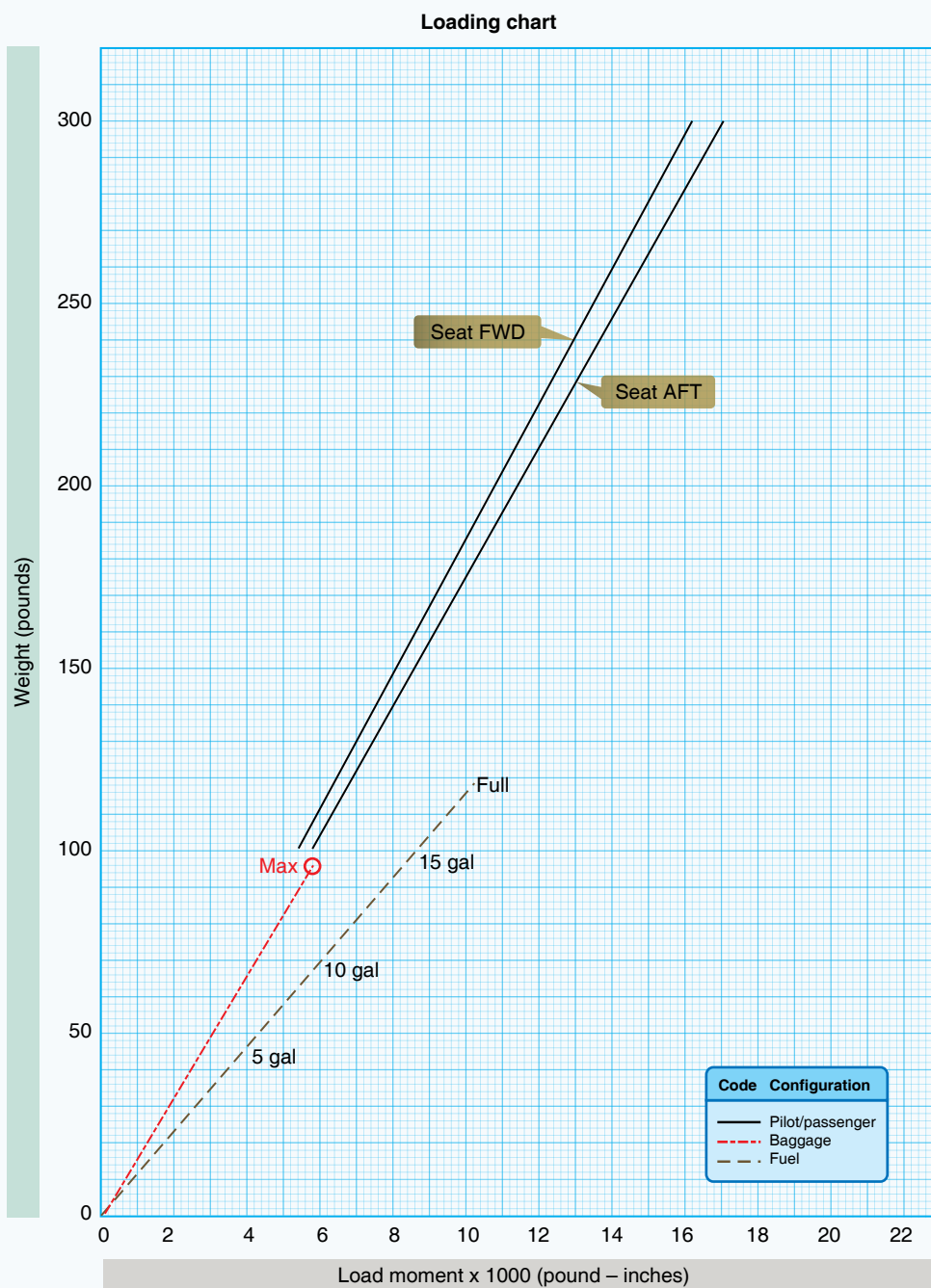
Figure 45. Gyroplane Weight and Balance Graph.
