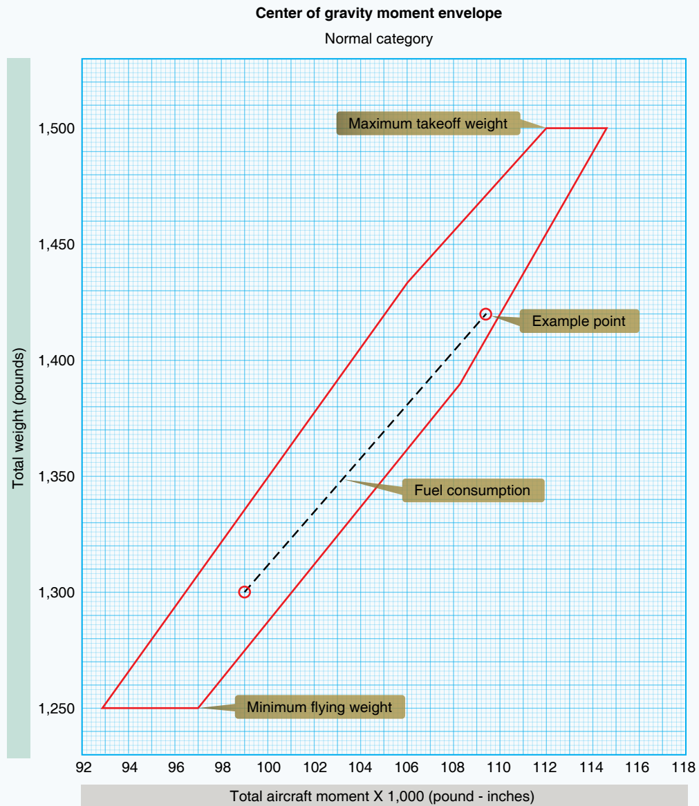
Figure 44. Gyroplane Weight and Balance Graph.
