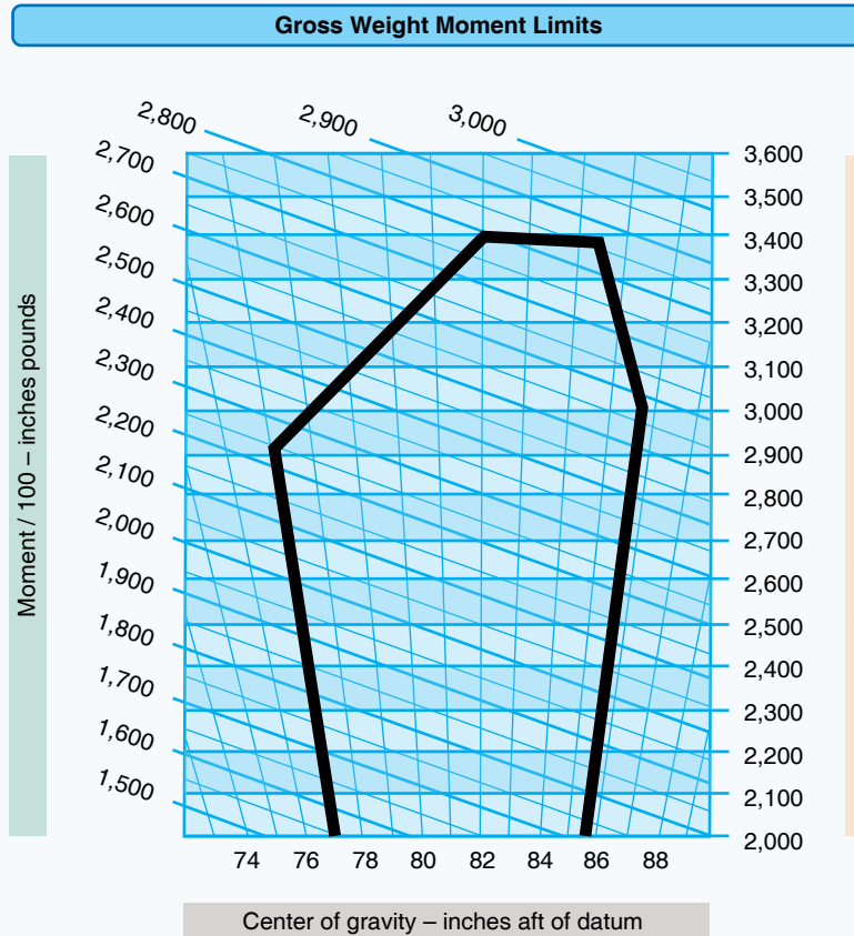
Figure 67. Weight and Balance Chart.
