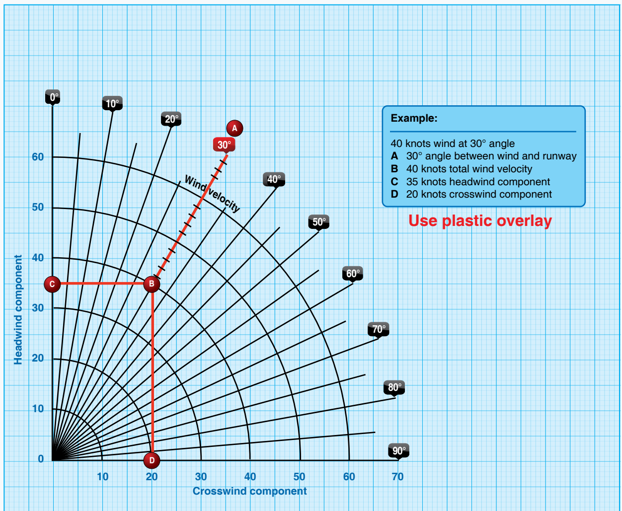
Figure 36. Crosswind Component Graph.
