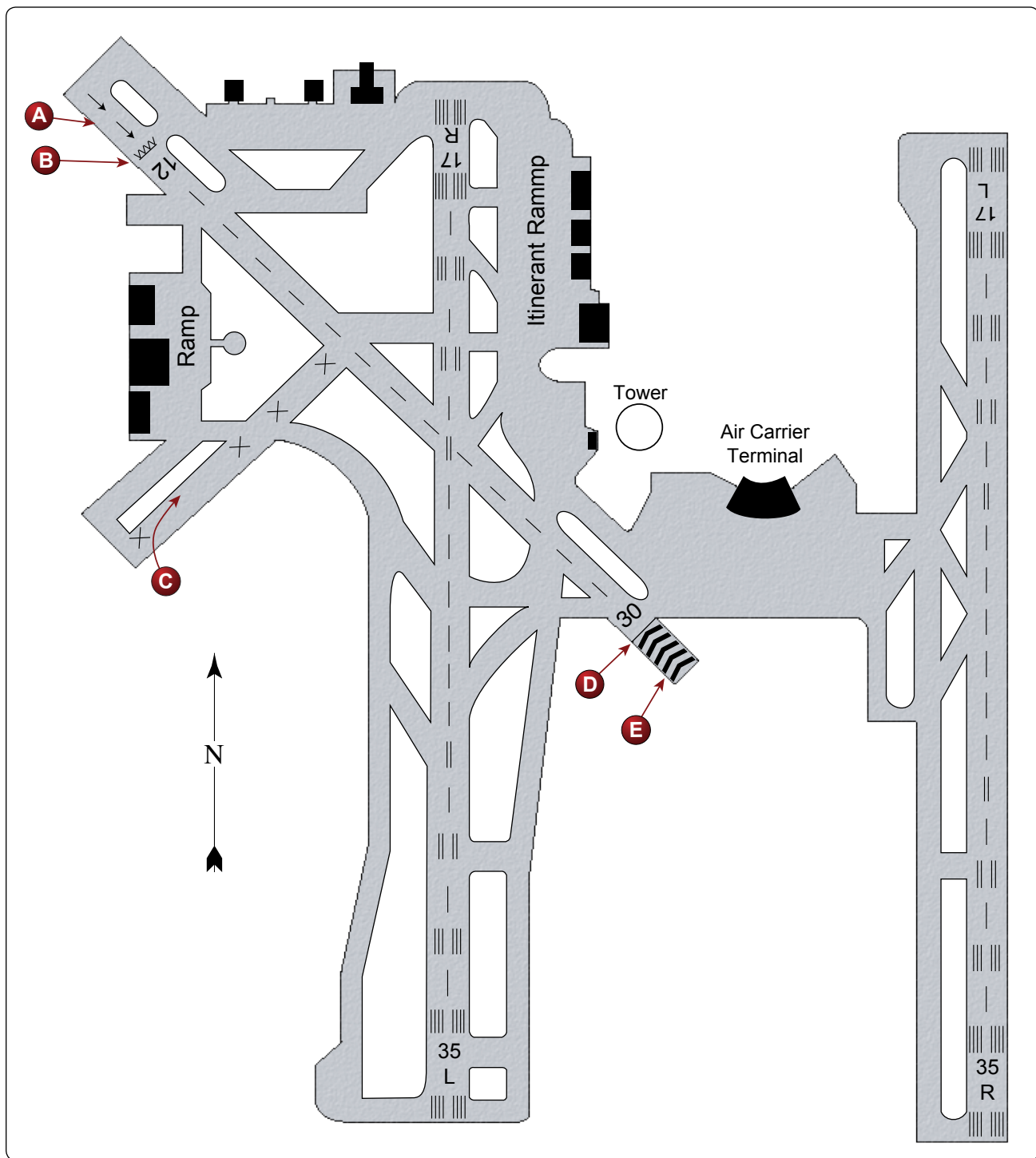
Figure 48. Airport Diagram.
