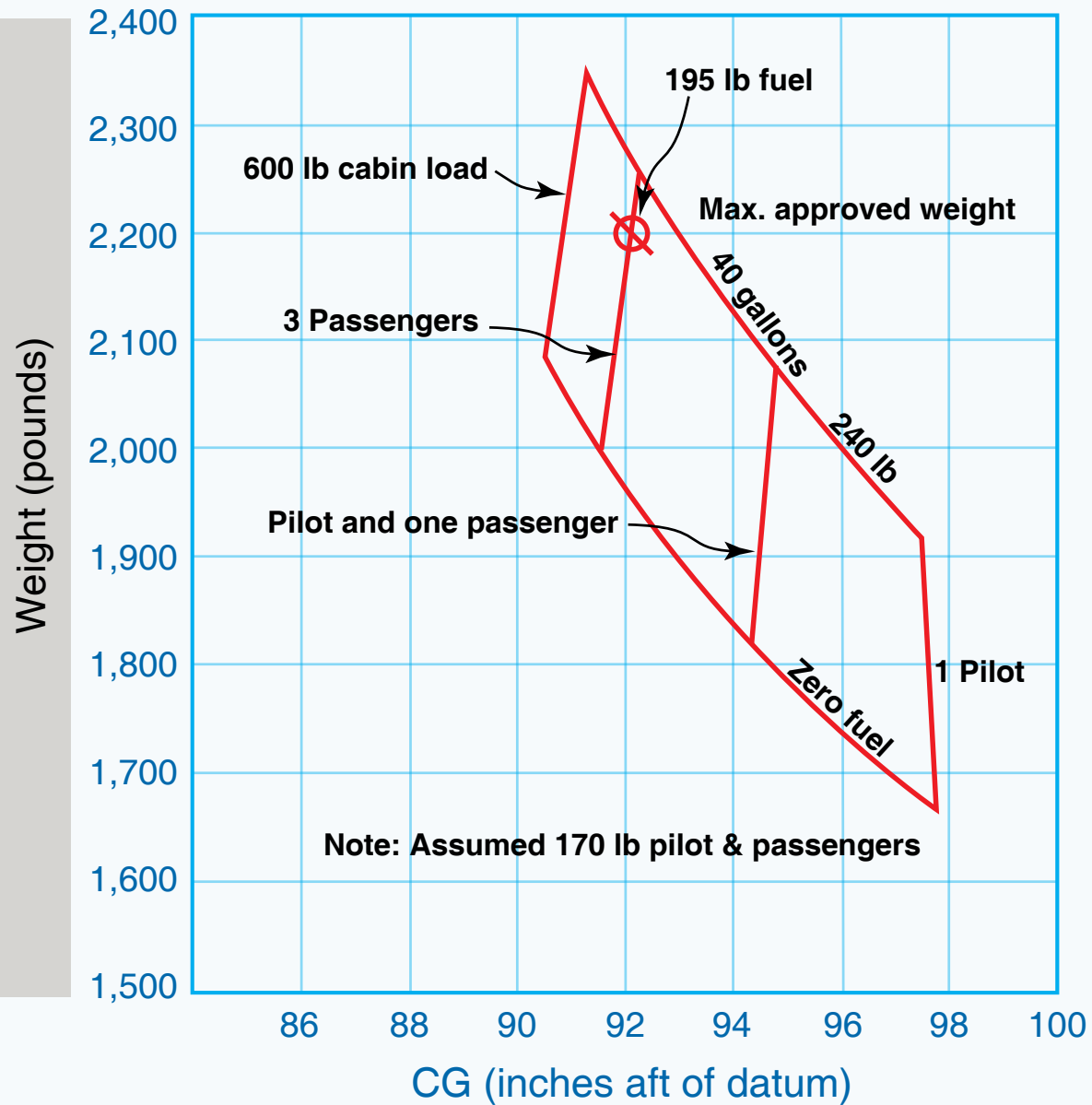
Figure 41. Helicopter Weight and Balance Graph.
