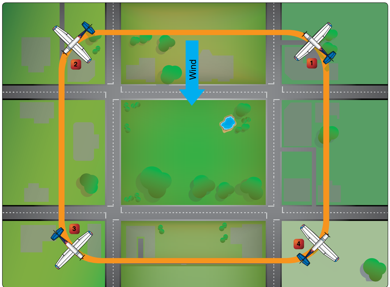
Figure 62. Rectangular Course.
