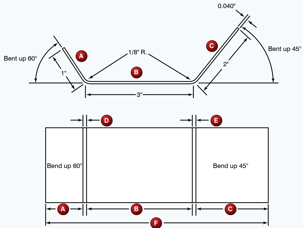
Figure 7. Sheet metal layout.
