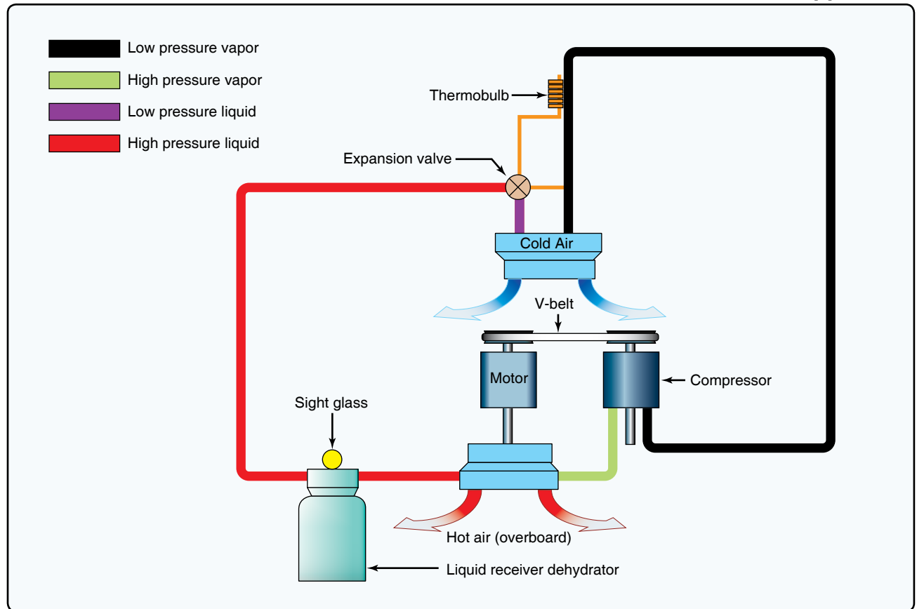
Figure 13. Cooling system.
