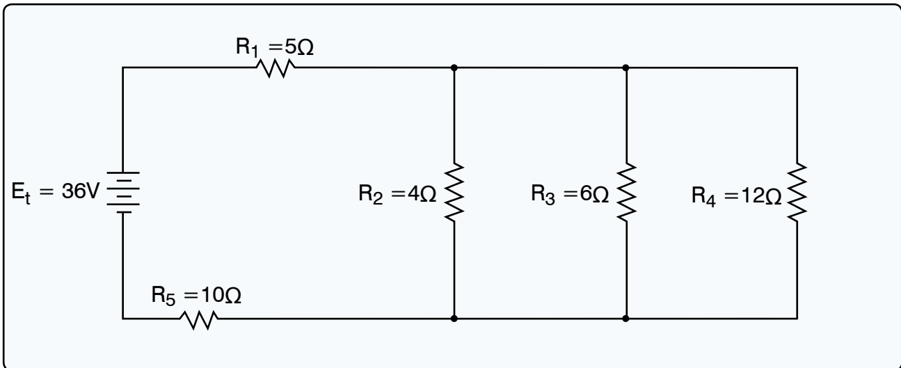
Figure 14. Circuit diagram.
