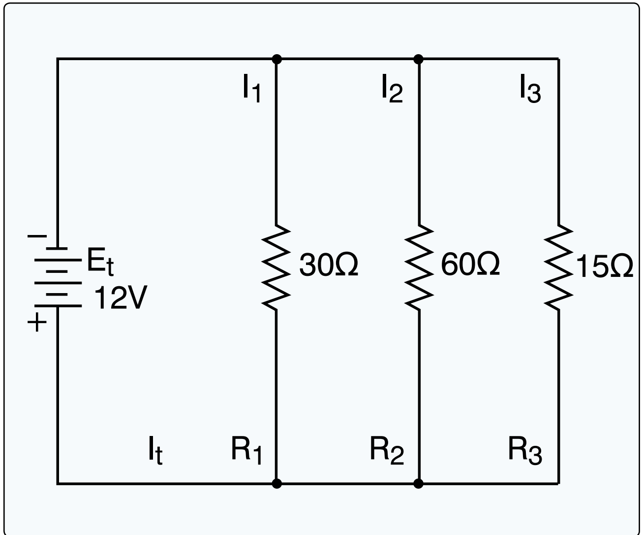
Figure 13. Circuit diagram.
