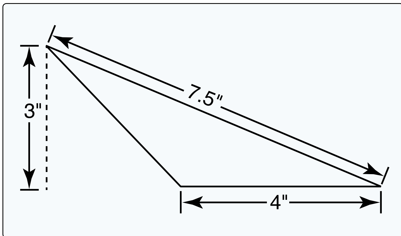
Figure 55. Triangle area.
