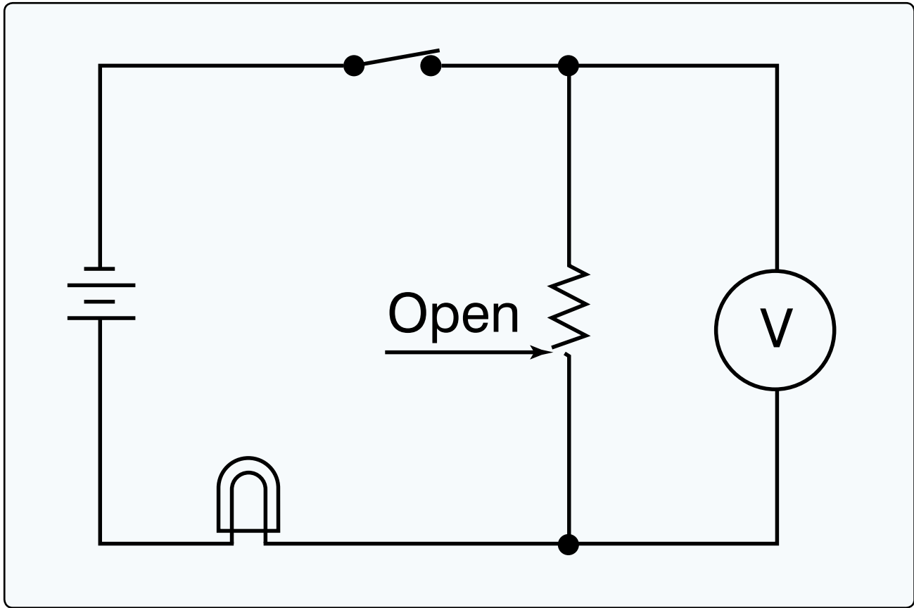
Figure 20. Circuit diagram.
