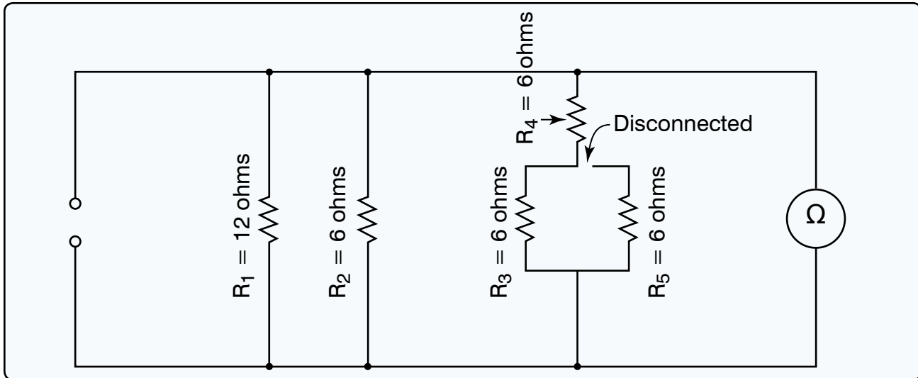
Figure 6. Circuit diagram.
