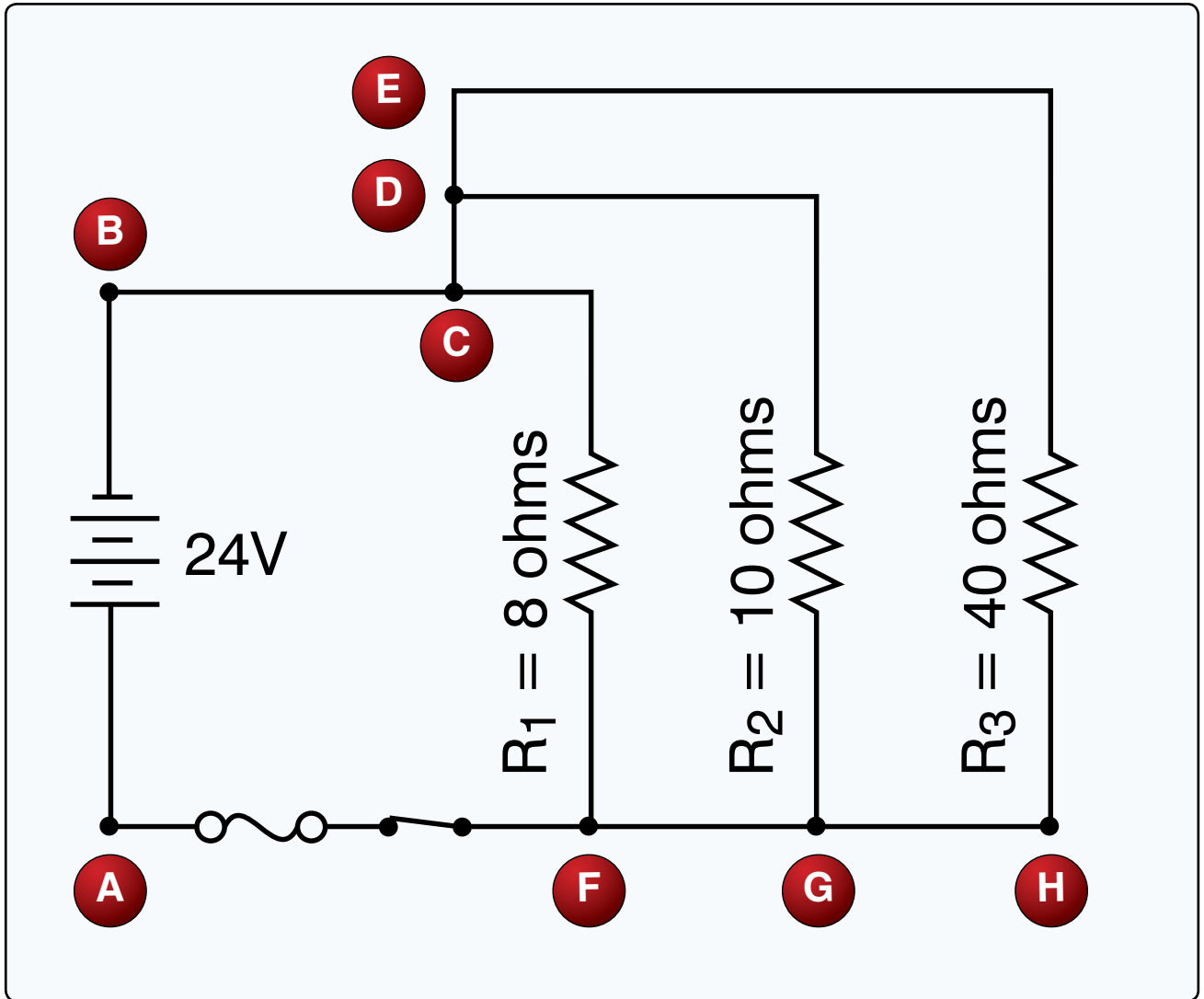
Figure 11. Circuit diagram.
