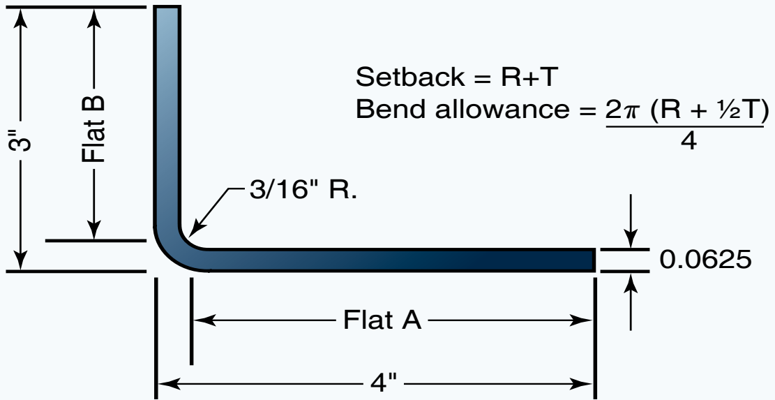
Figure 4. Bending sheet metal.
