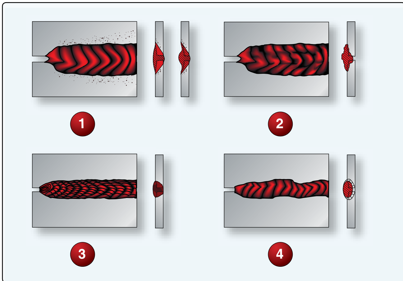
Figure 44. Welds.
