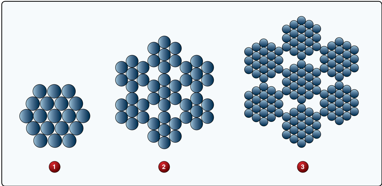
Figure 8. Control cable.
