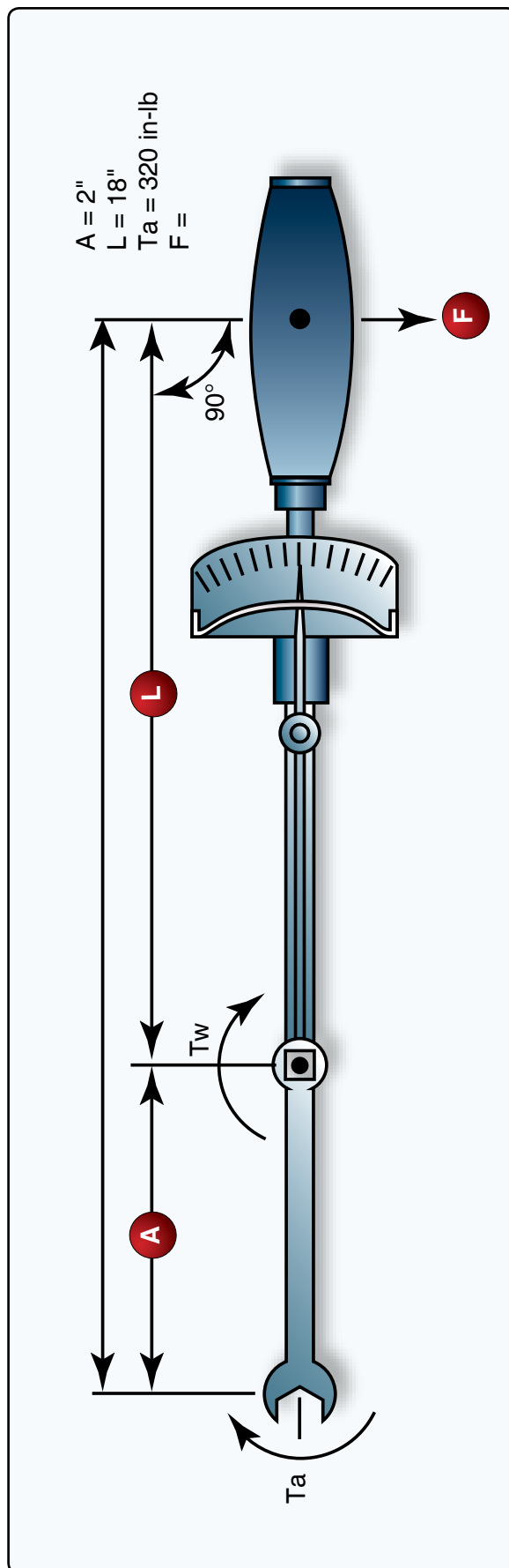
Figure 10. Torque value.
