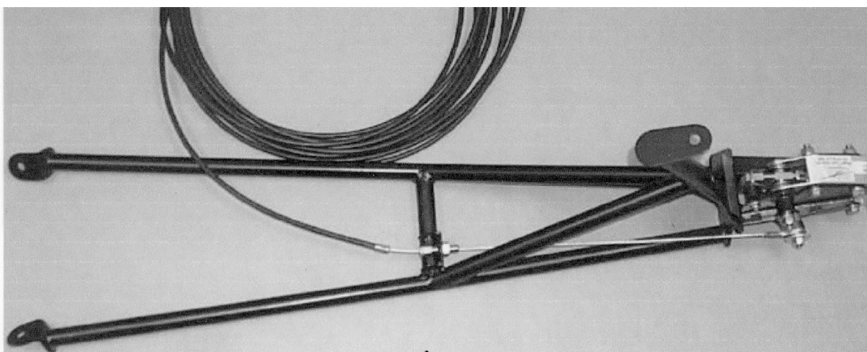
Figure 9-12. Typical TOST Mount for Tricycle Gear Aircraft
