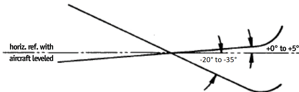
Figure 6-6. Main Ski Incidence Angles
