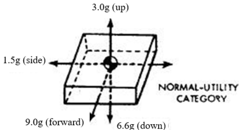
Figure 3-1. Force Diagram Normal-Utility Category
