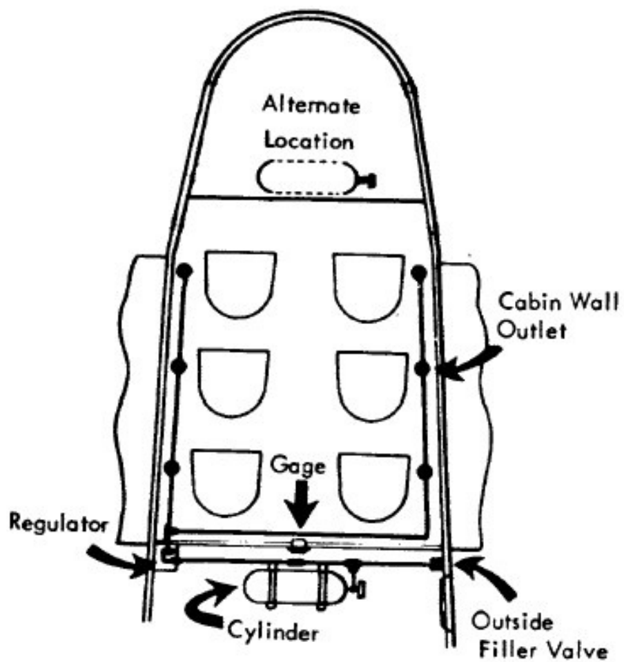
Figure 7-3. Typical Oxygen Installation in Light Twin Aircraft
