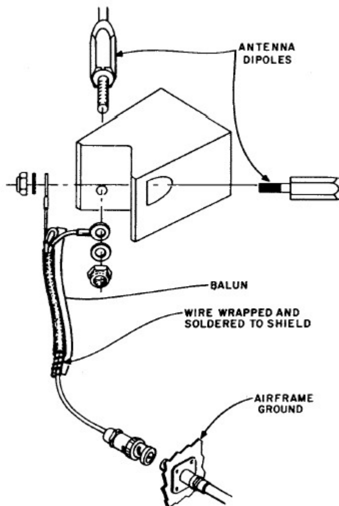
Figure 4-5. Typical Dipole Antenna Assembly
