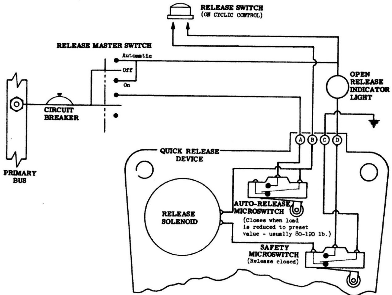
Figure 8-2. Typical Cargo Sling Wiring Diagram
