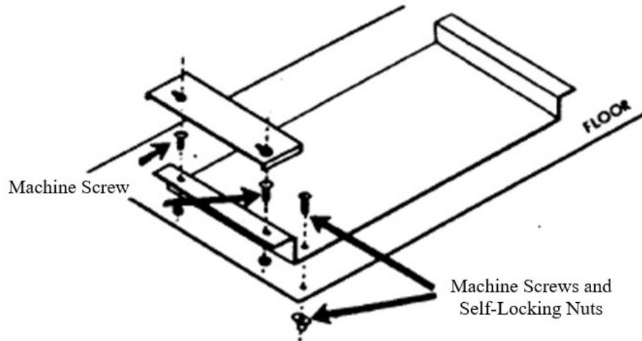
Figure 3-6. Typical Rigid Base Plate Mount
