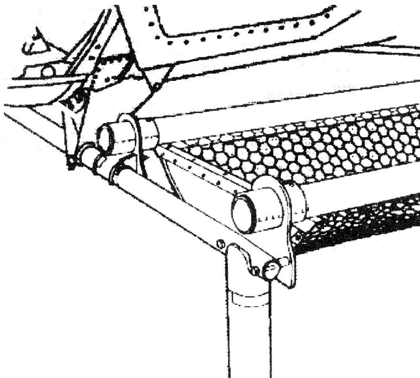
Figure 8-11. Typical Cargo Rack Installation No. 1 (Showing Attachment Detail)
