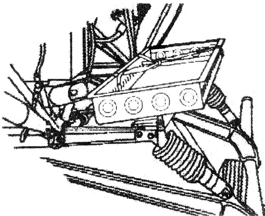
Figure 8-12. Typical Cargo Rack Installation No. 2
