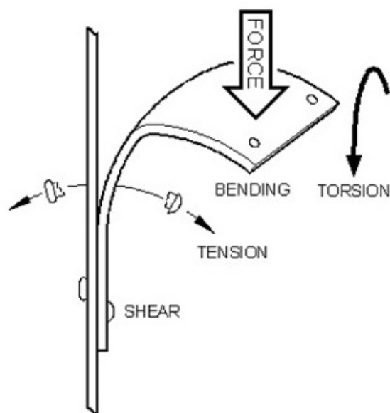
Figure 2-2. Typical Load
