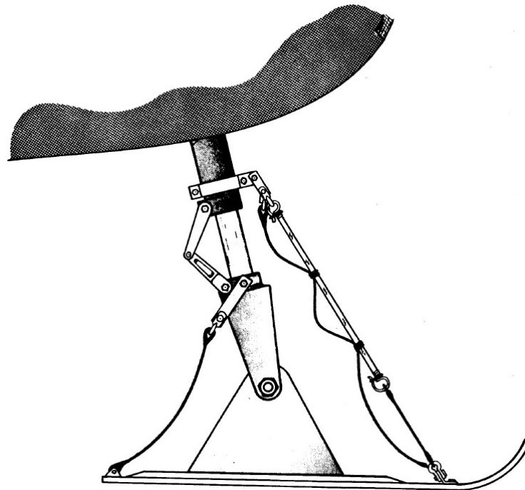
Figure 6-7. Typical Nose Ski Installation
