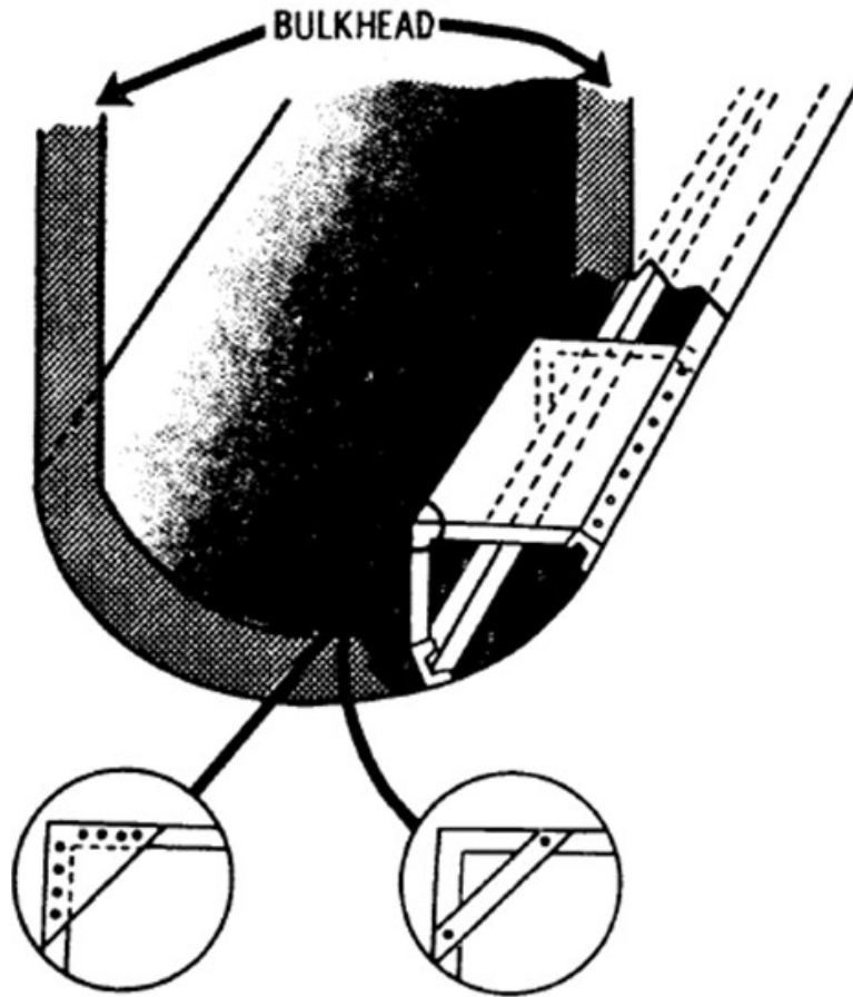
Figure 3-9. Typical Shelf Installation
