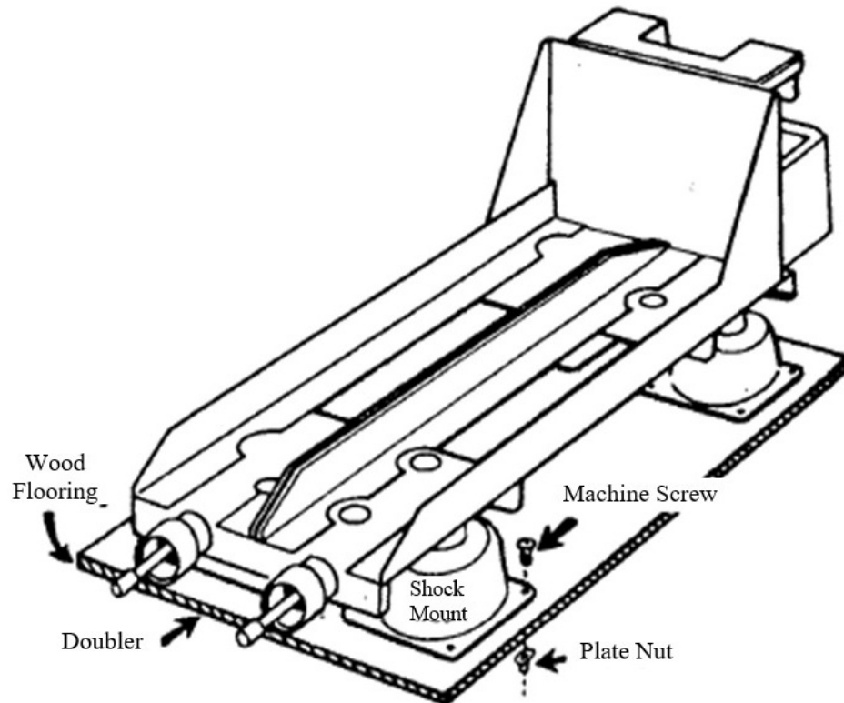
Figure 3-4. Typical Shock-Mounted Base (Wood or Composition Flooring)
