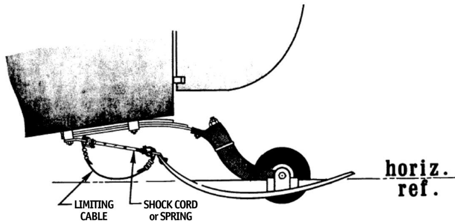
Figure 6-8. Typical Tail Ski Installation
