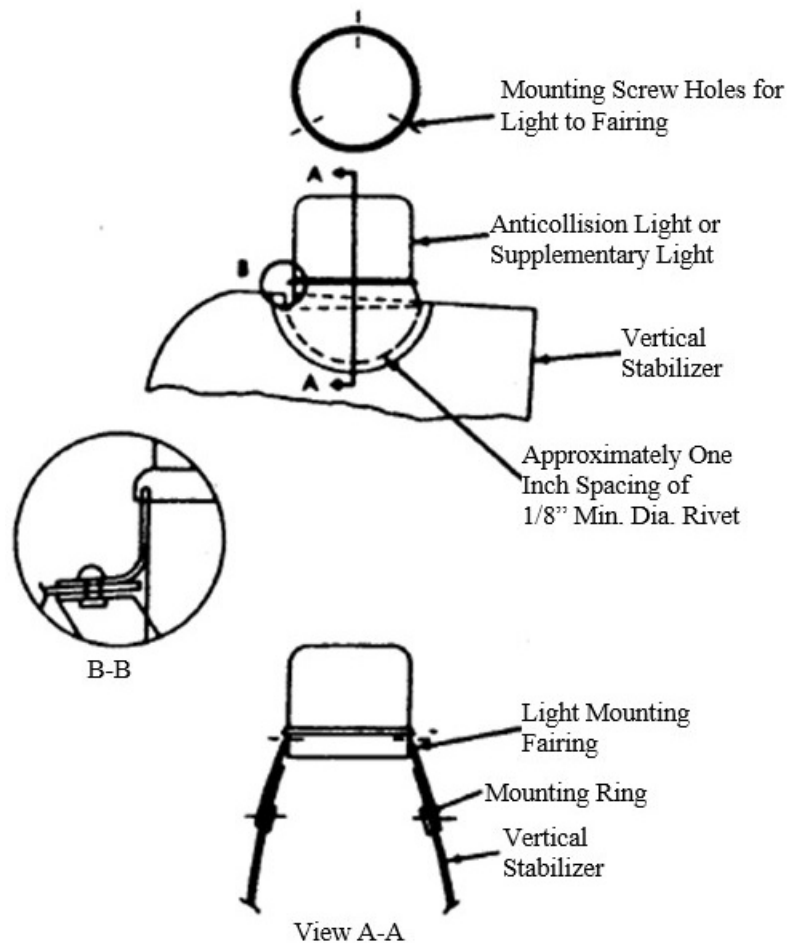
Figure 5-3. Typical Anticollision or Supplementary Light Installation in a Fin Tip
