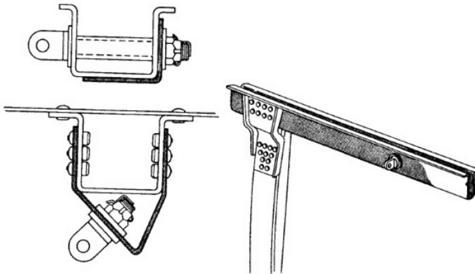
Figure 10-14. Typical Wing Carry-Through Installation
