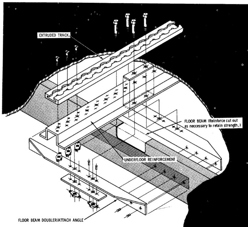
Figure 13-4. Installation of Underfloor Support for Extruded Track
