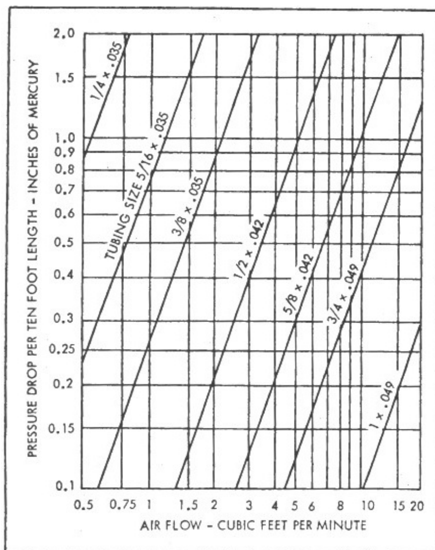
Figure 12-2. Pressure Drop Data for Smooth Tubing
