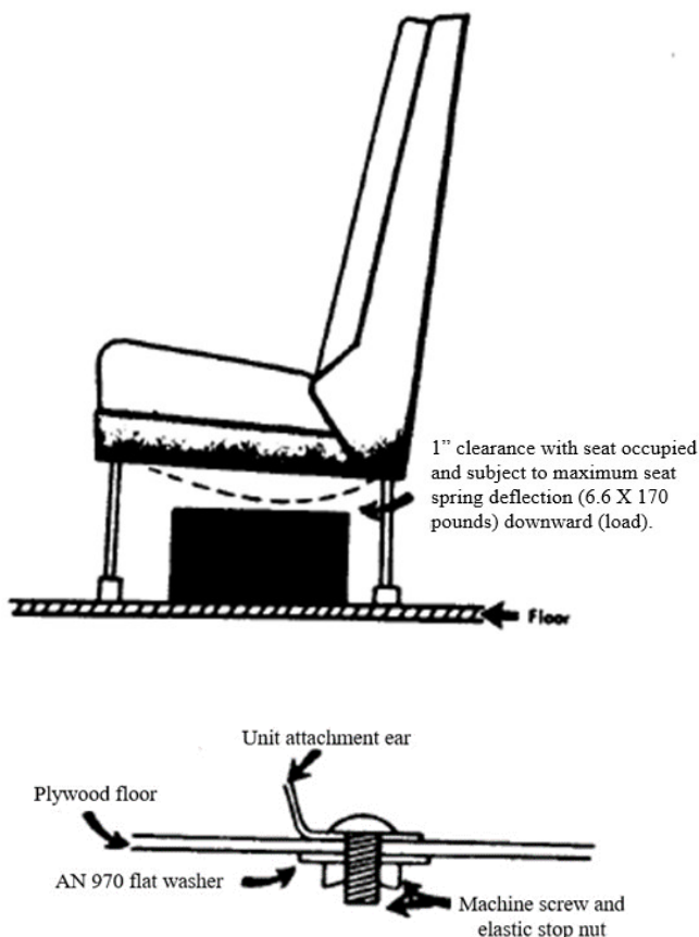
Figure 3-7. Typical Underseat Installation
