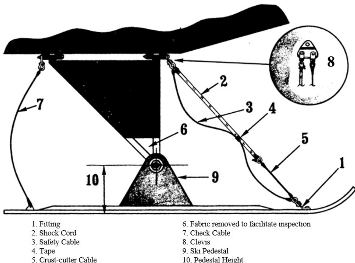
Figure 6-2. Typical Ski Installation
