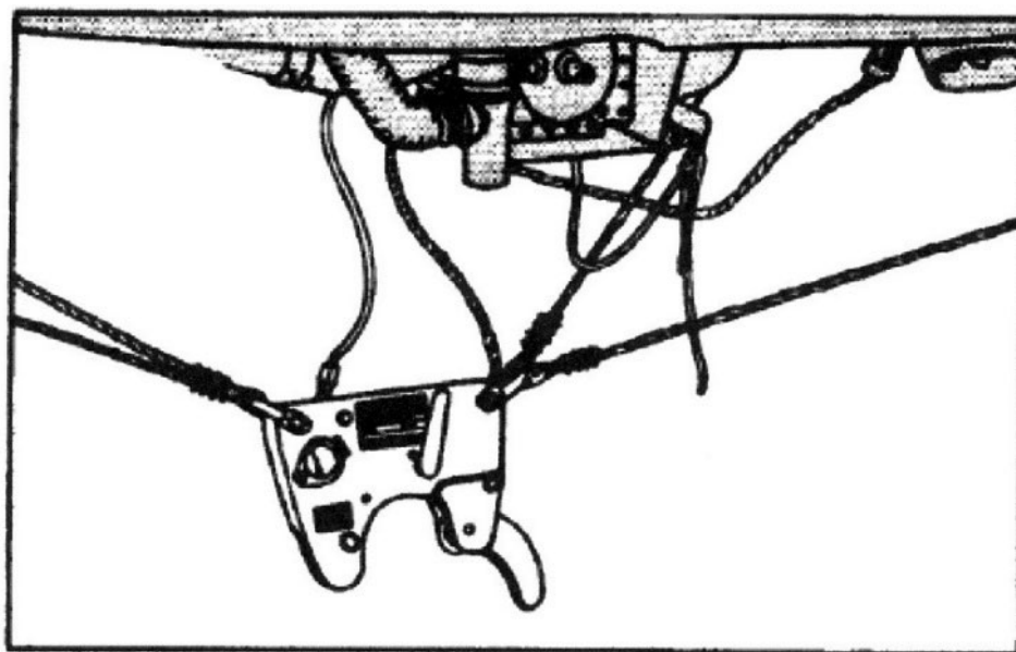
Figure 8-7. Typical Cargo Sling Installation No. 3 (4-Leg, Cable Suspended)
