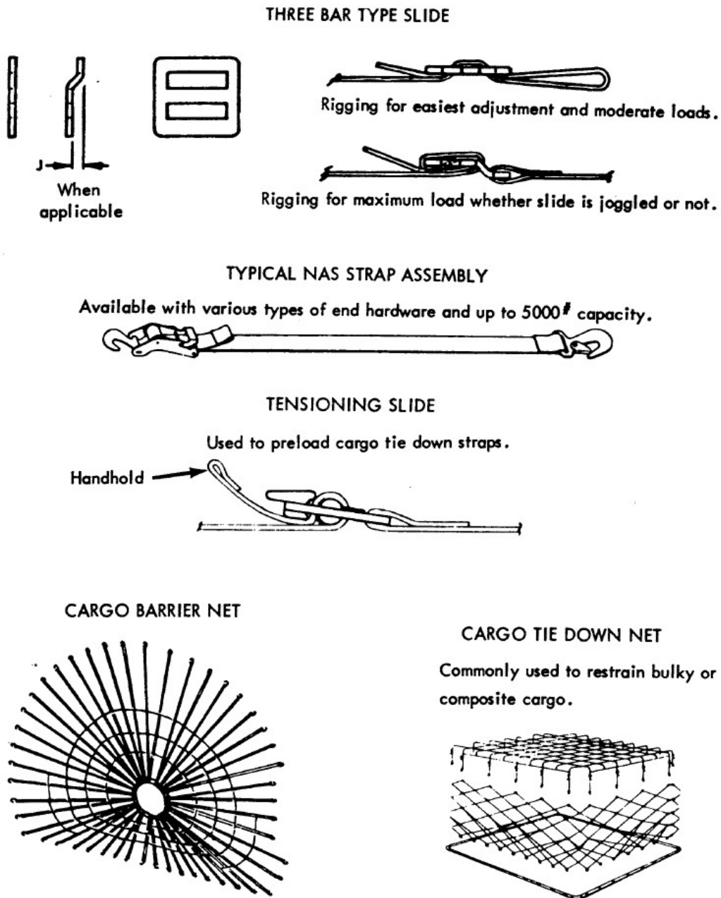
Figure 13-5. Typical Cargo Tiedown Straps and Cargo Nets
