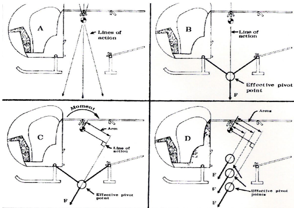
Figure 8-1. Location of Cargo Release in Relation to the Rotorcraft's Center of Gravity
