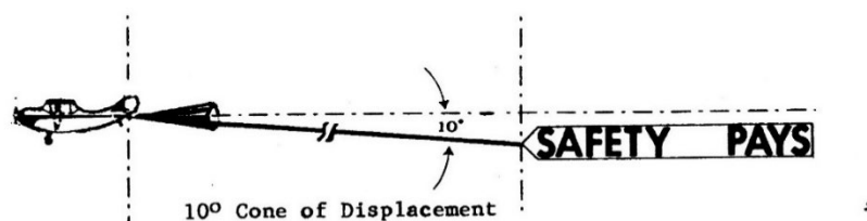
Figure 9-2. Banner Tow Angle
