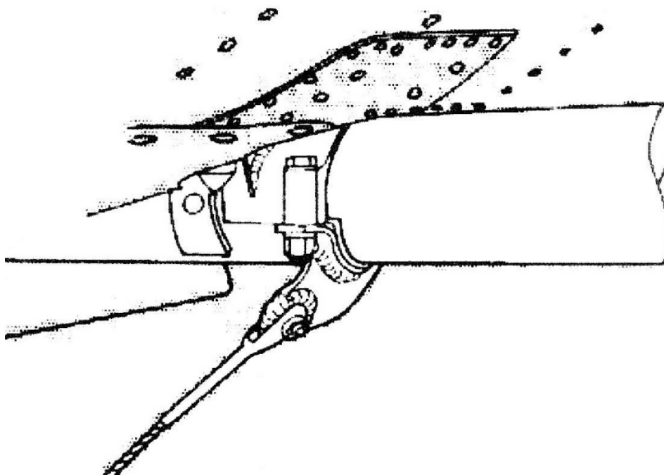
Figure 8-8. Typical Cargo Sling Installation No. 3 (Showing Cable Sling Leg Attachment to Landing Gear Crosstube Fitting)
