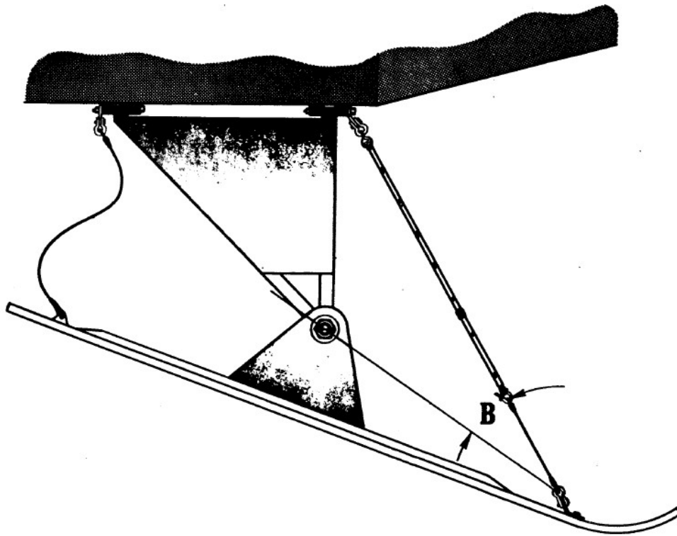
Figure 6-5. Main Ski at Maximum Negative Incidence (Safety Cable Taut)
