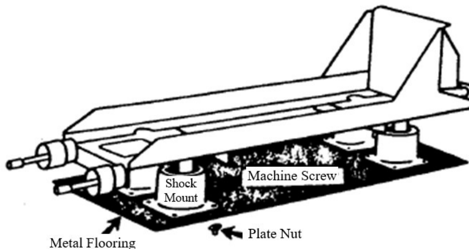
Figure 3-5. Typical Shock-Mounted Base (Metal Flooring)
