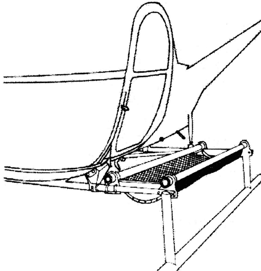
Figure 8-10. Typical Cargo Rack Installation No. 1
