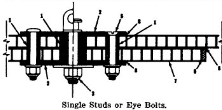
Figure 13-3. Typical Attachment of Fittings to Honeycomb Structures
