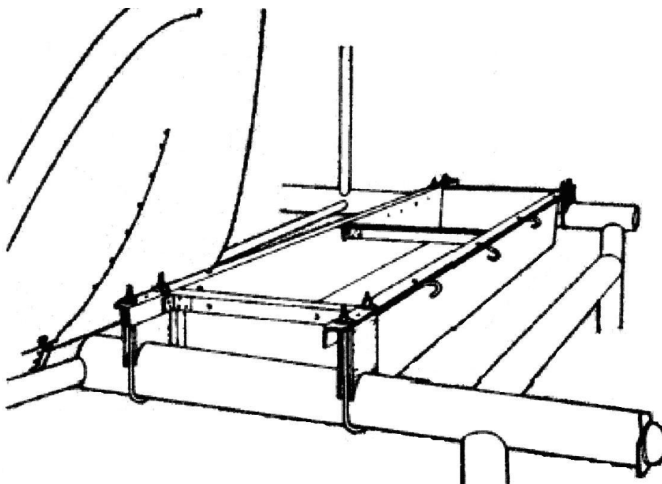
Figure 8-14. Typical Cargo Rack Installation No. 3
