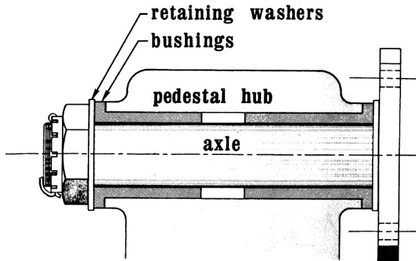
Figure 6-1. Typical Hub Installation
