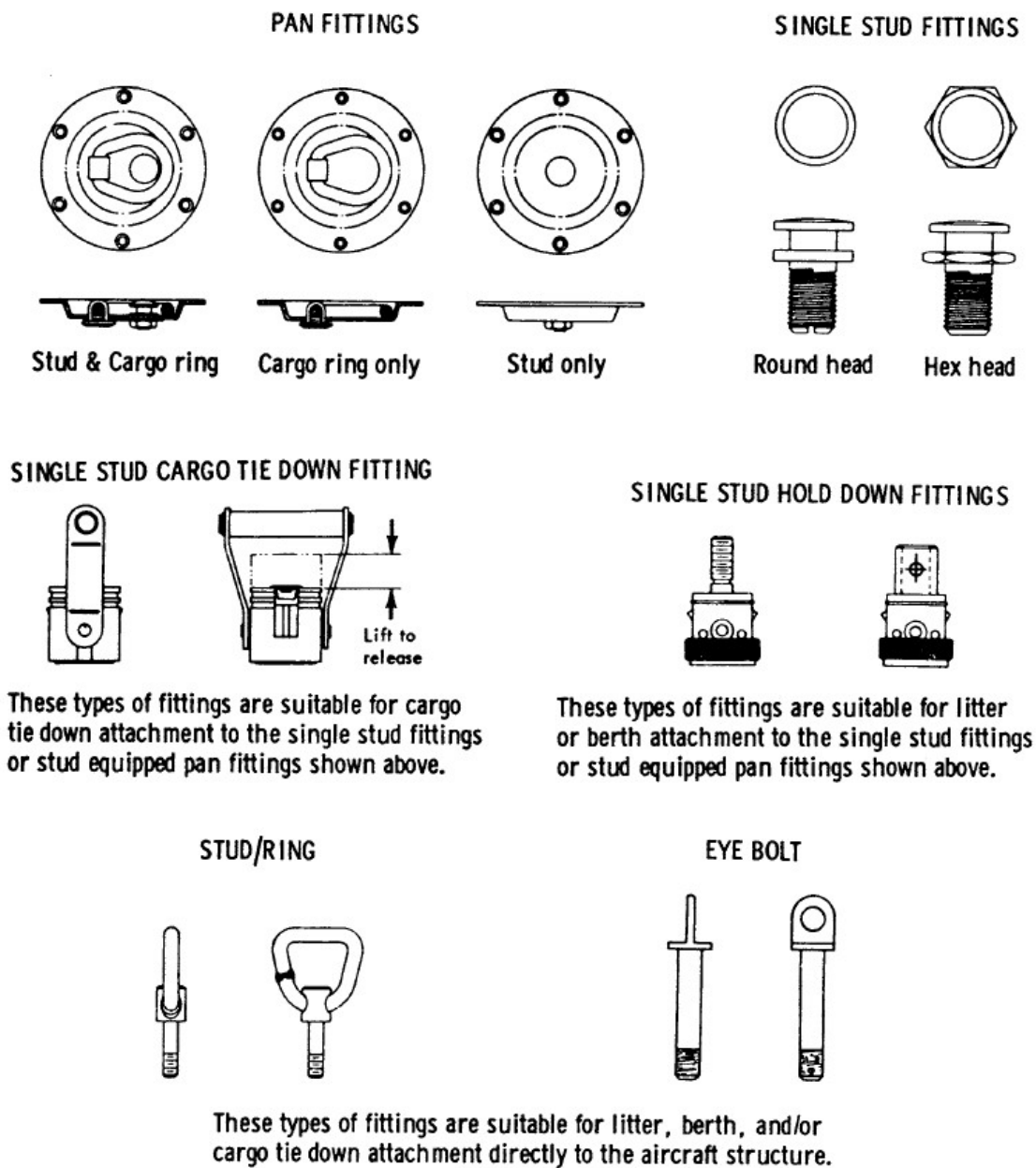
Figure 13-2. Miscellaneous Litter, Berth, and Cargo Tiedown Fittings
