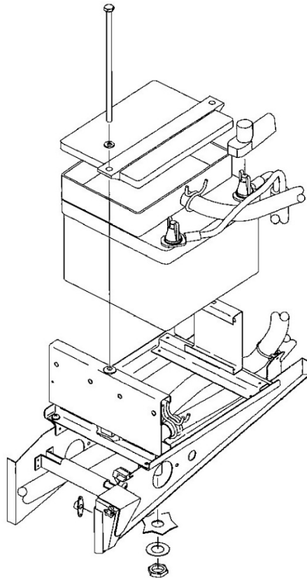
Figure 11-1. Typical Battery Installation in the Aircraft
