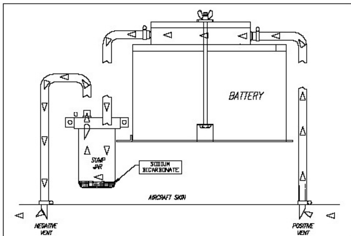
Figure 11-3. Battery Ventilation System
