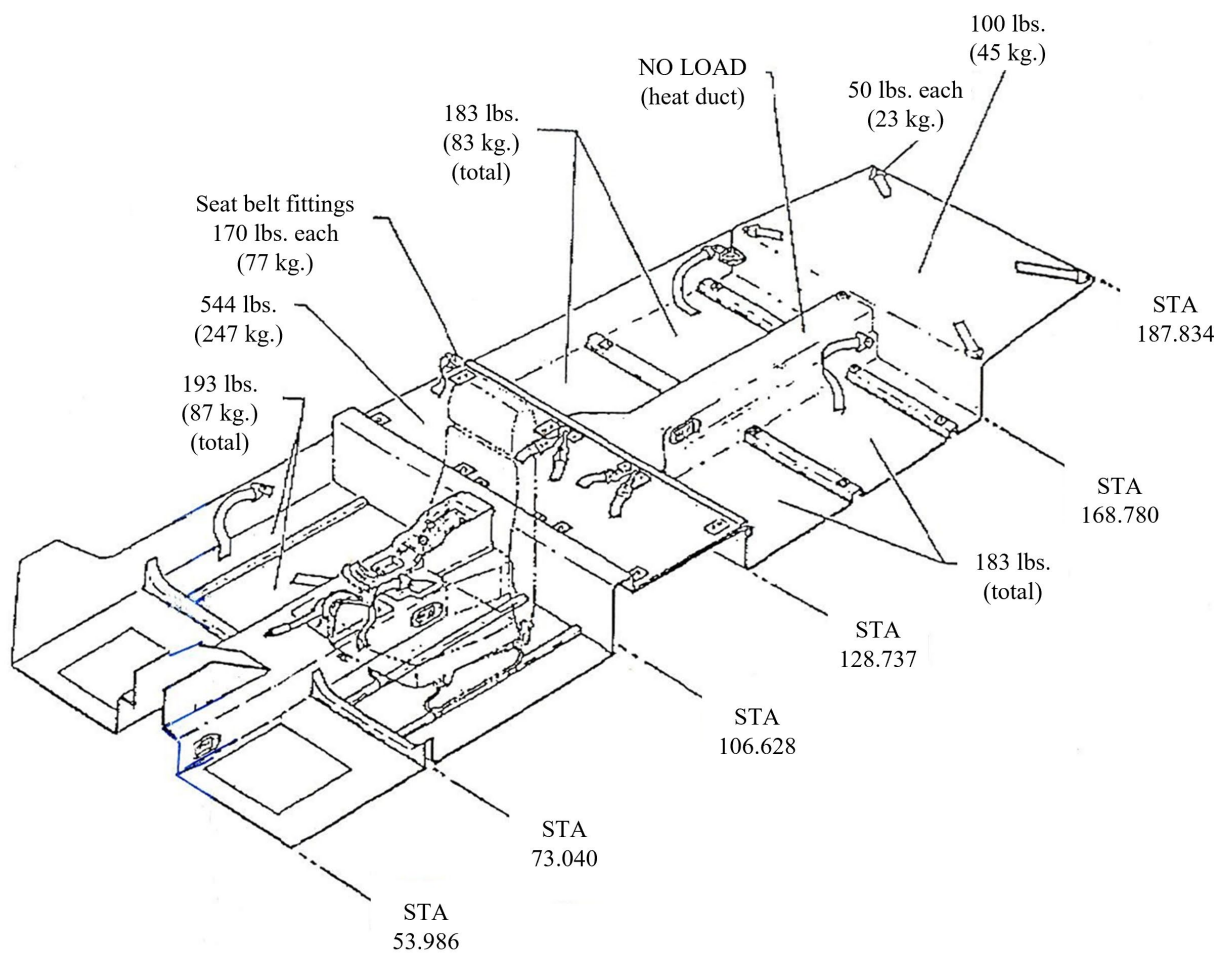
Figure 13-6. Example of Allowable Cargo Loading Diagram
