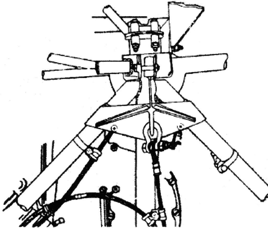
Figure 8-4. Typical Cargo Sling Installation No. 1 (Showing Fuselage Attachment Fitting)
