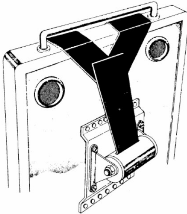
Figure 10-13. Typical Seat Mounted Inertia Reel Installation
