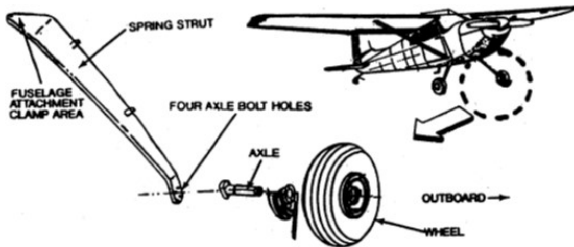
Figure 14-2. Typical Main Landing Gear Spring Strut and Axle Assembly
