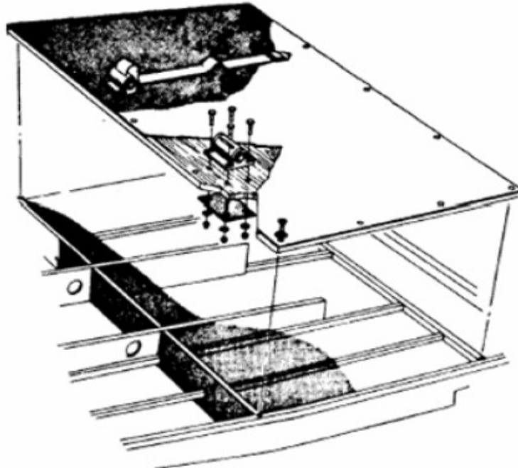
Figure 10-12. Typical Floor Mounted Inertia Reel Installation
