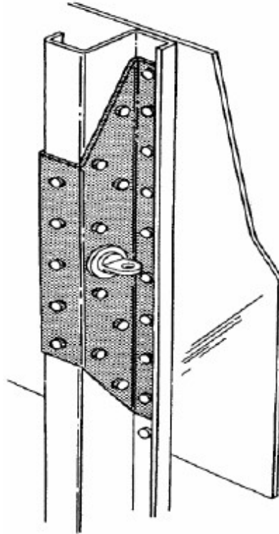
Figure 10-19. Typical Attachments to Tubular Members
