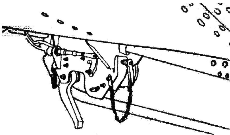
Figure 8-6. Typical Cargo Sling Installation No. 2 (Cargo Hook Attached Directly to Underside of Fuselage)
