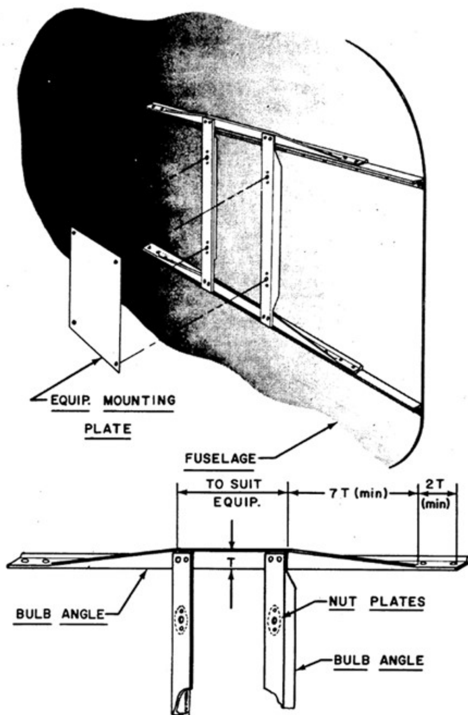
Figure 3-8. Typical Remote Unit Mounting Base-Vertical or Horizontal Other Than Structure to Floor
