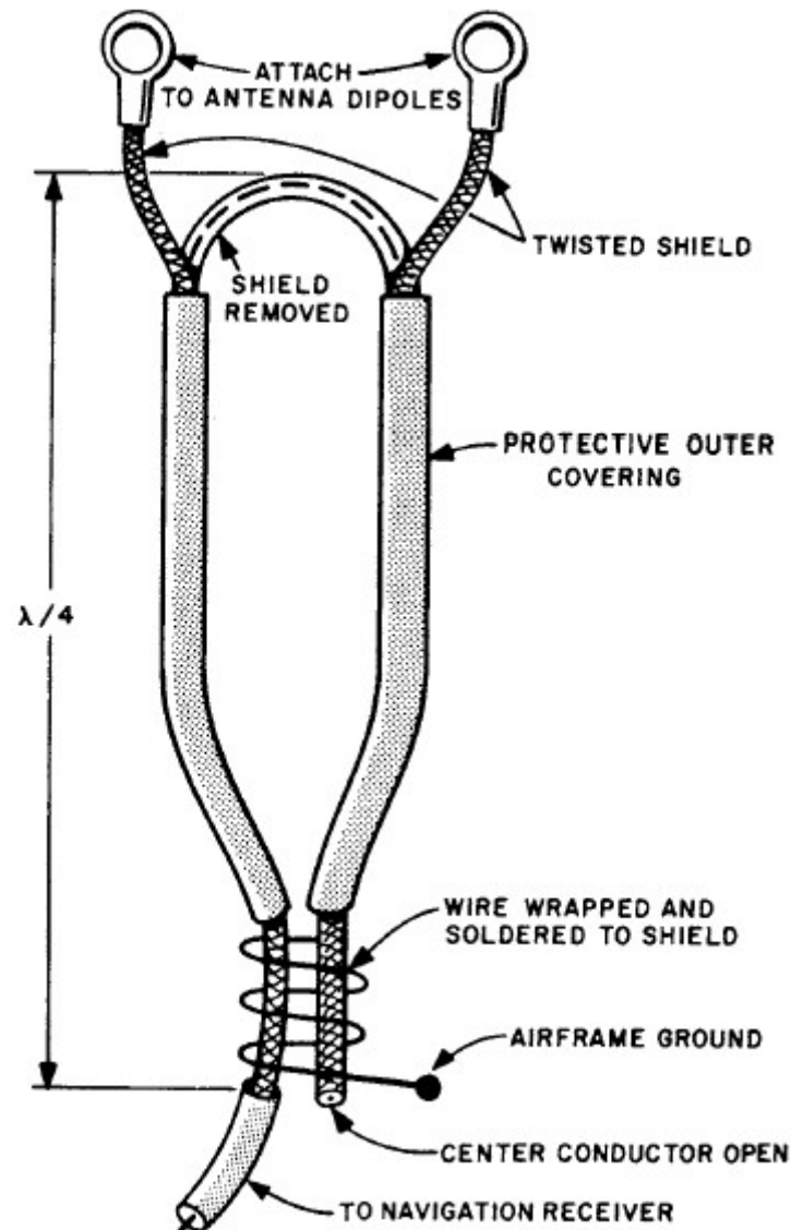
Figure 4-6. Typical VOR Balun
