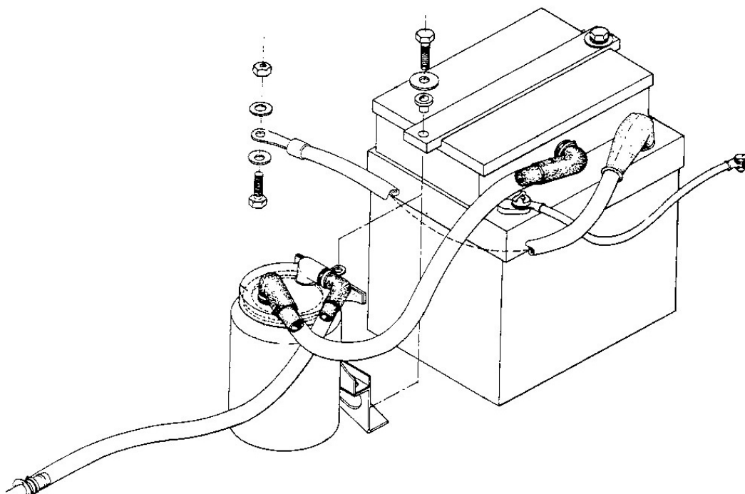
Figure 11-2. Typical Battery Installation With Sump Jar
