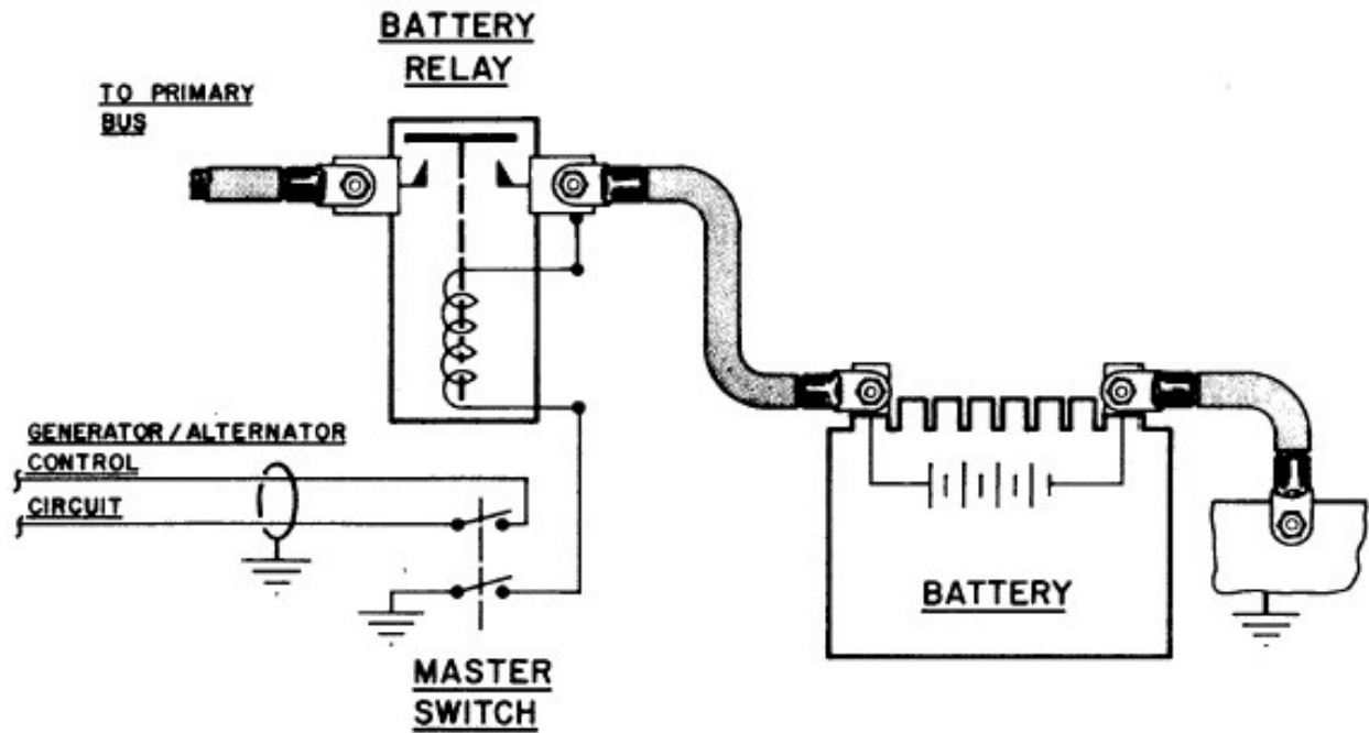
Figure 11-4. Typical Battery Cutoff and Generator Alternator Control Circuit
