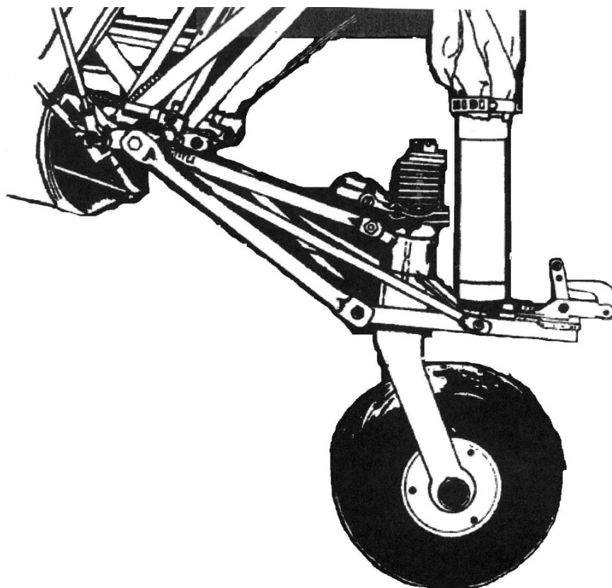
Figure 9-6. Conventional Gear Aircraft—Shock Strut Type Tailwheel
