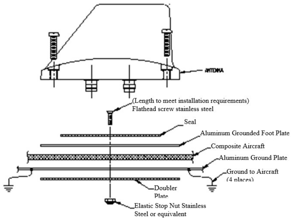
Figure 4-3. One Means to Provide Adequate Antenna Bonding Through a Composite Airframe
