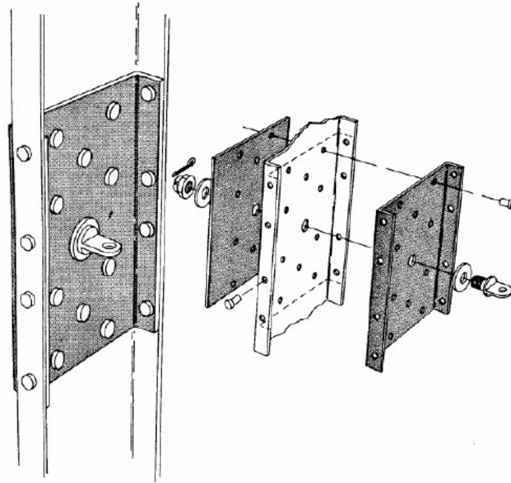
Figure 10-16. Typical Bulkhead Reinforcement Installation
