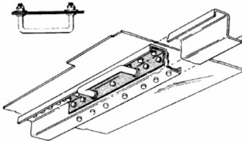
Figure 10-17. Typical Stringer Section Reinforcement Installation
