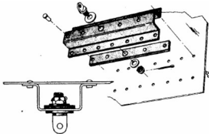
Figure 10-15. Typical Hat Section Reinforcement Installation
