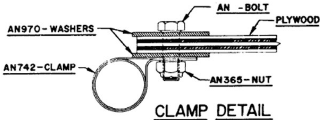
Figure 3-10. Typical Attachment of Support Structure to Tubular Frame Other Than Structure to Floor
