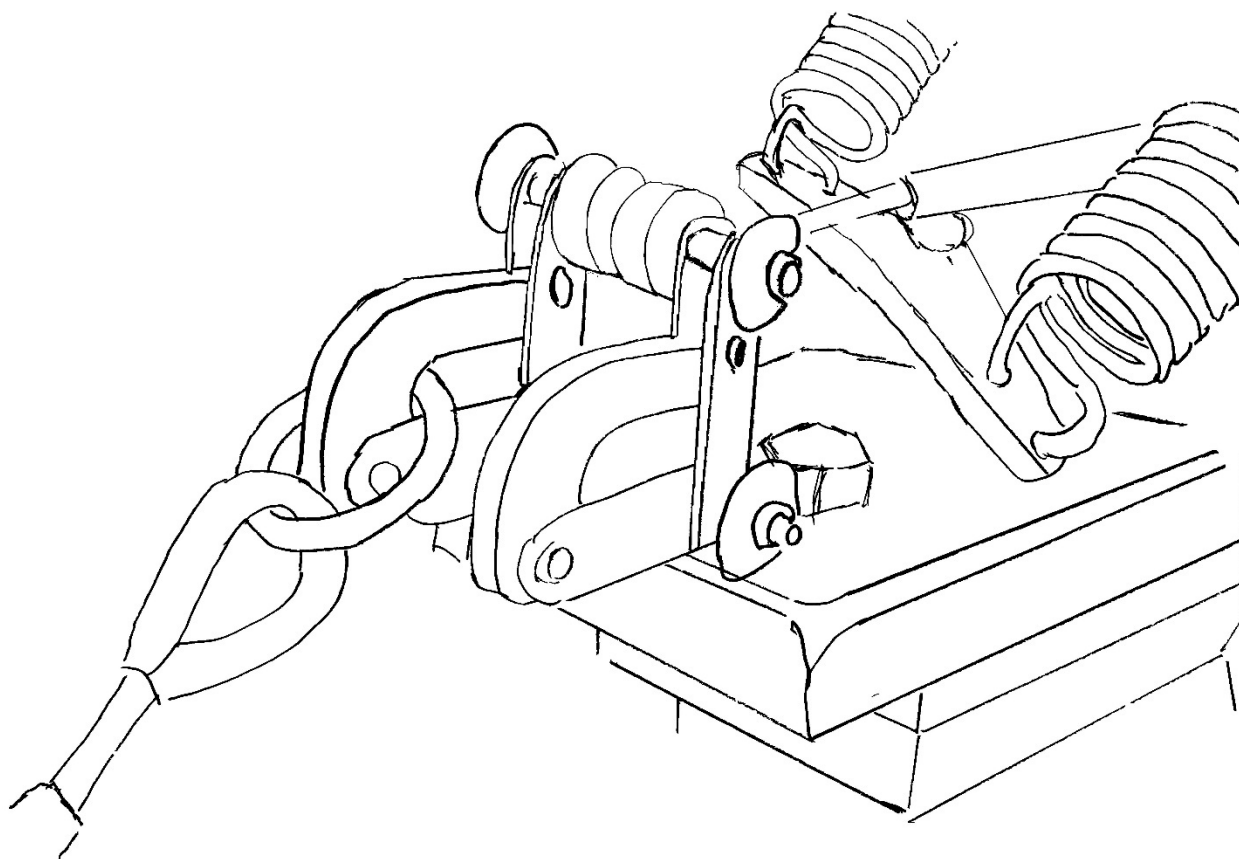
Figure 9-11. Typical Multiple Hitch for Banner Tow
