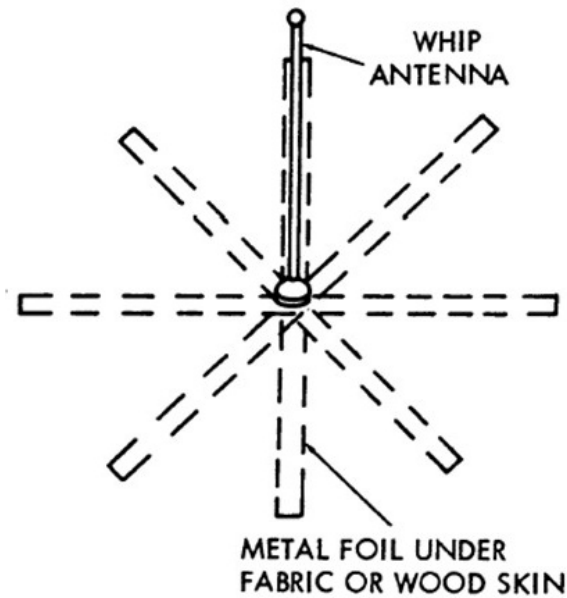
Figure 4-2. Antenna Ground Plane for Nonconductive Mount
