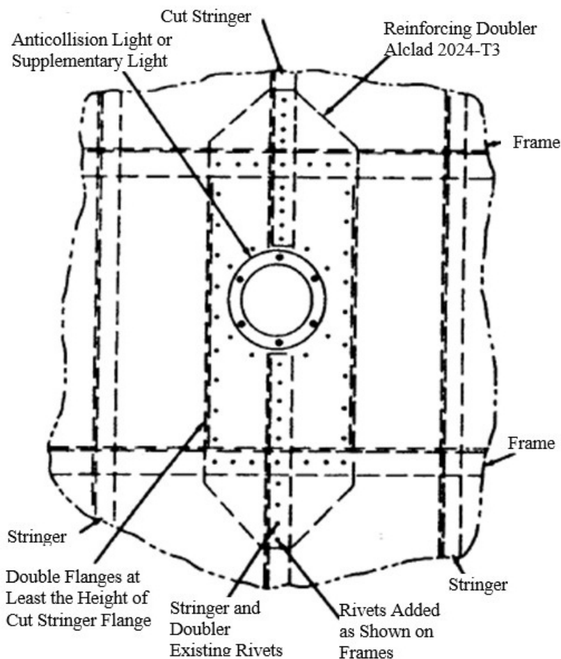
Figure 5-2. Typical Anticollision or Supplementary Light Installation Involving a Cut Stringer (Unpressurized)
