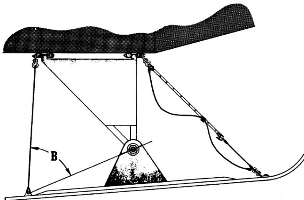
Figure 6-4. Main Ski at Maximum Positive Incidence (Check Cable Taut)
