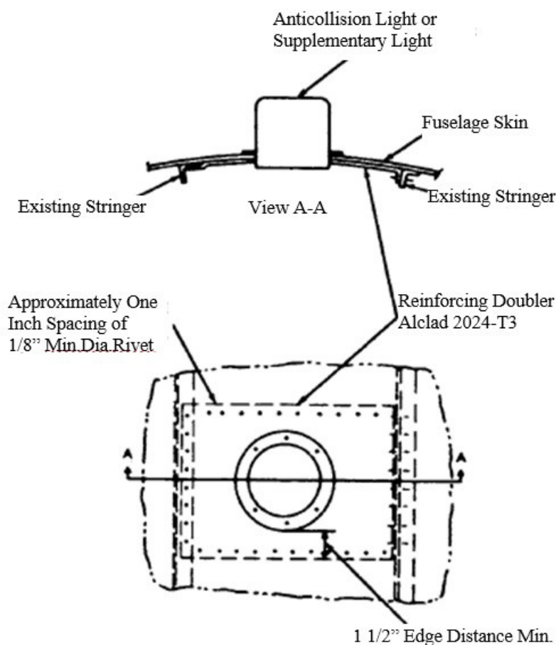
Figure 5-1. Typical Anticollision or Supplementary Light Installation in a Skin Panel (Unpressurized)
