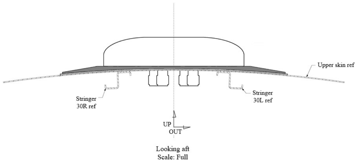
Figure 4-1. Antenna Mount With Saddle
