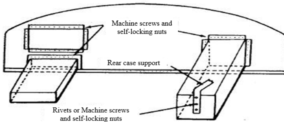
Figure 3-2. Typical Fabricated Panel Mounting
