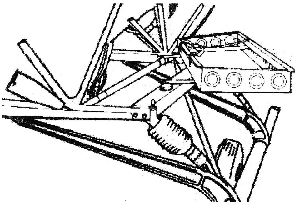
Figure 8-13. Typical Cargo Rack Installation No. 2 (Showing Rack Partially Installed)
