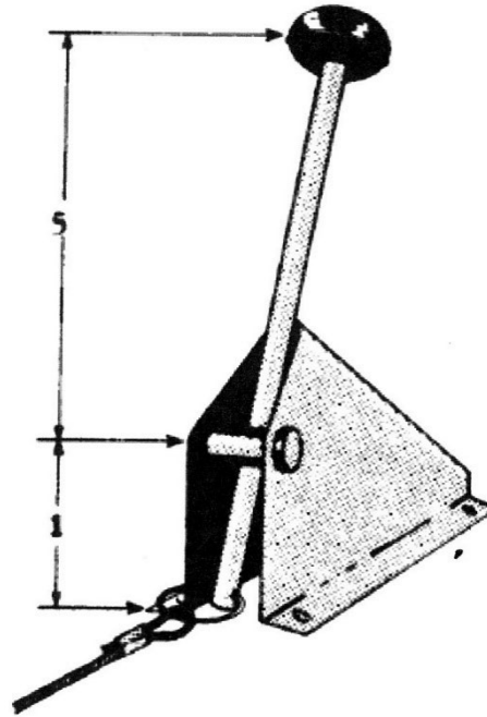
Figure 9-3. Typical Tow-Hitch Release Handle
