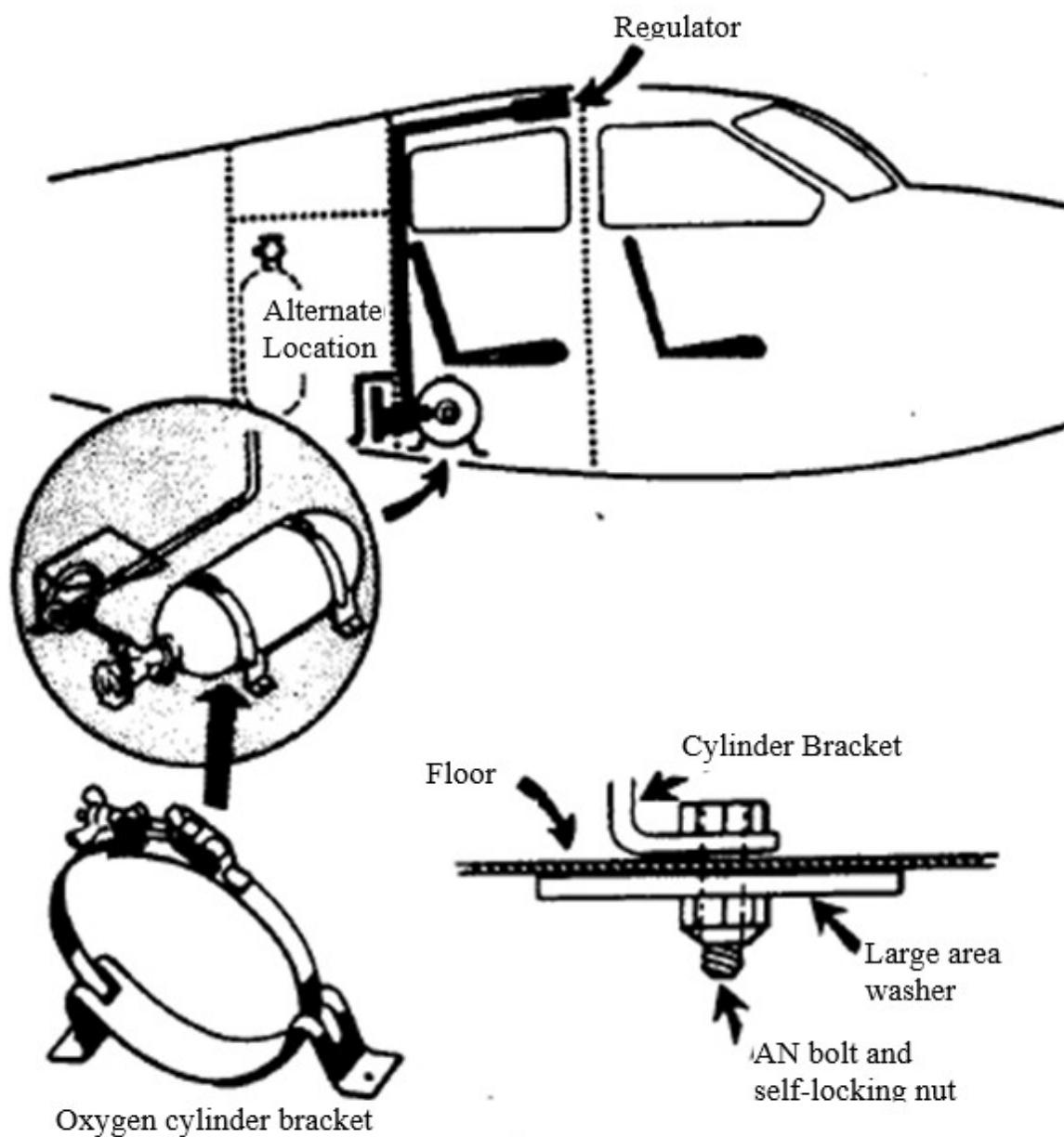
Figure 7-1. Typical Floor Mounting
