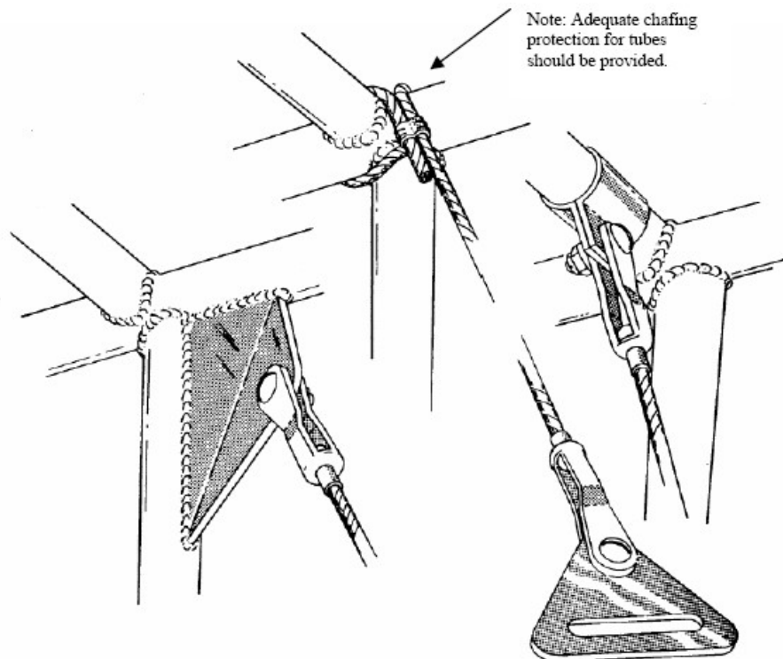
Figure 10-19. Typical Attachments to Tubular Members
