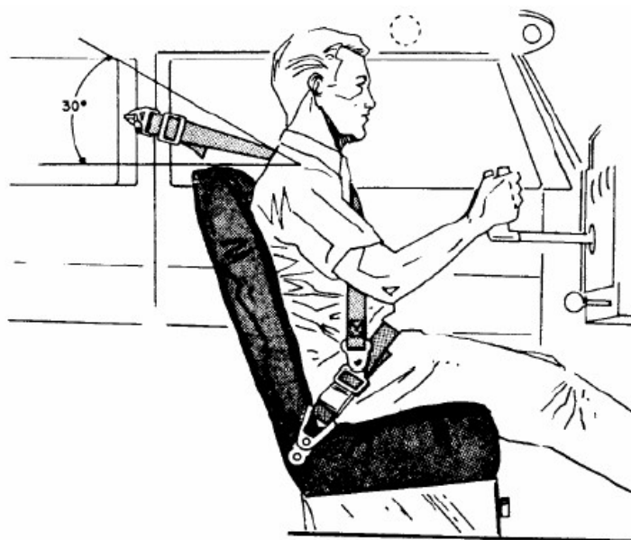
Figure 10-3. Side Mounted Single Diagonal Type Harness
