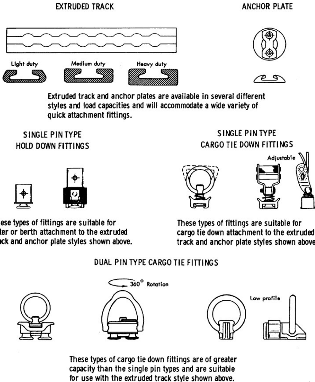
Figure 13-1. Extruded Track, Anchor Plates, and Associated Fittings
