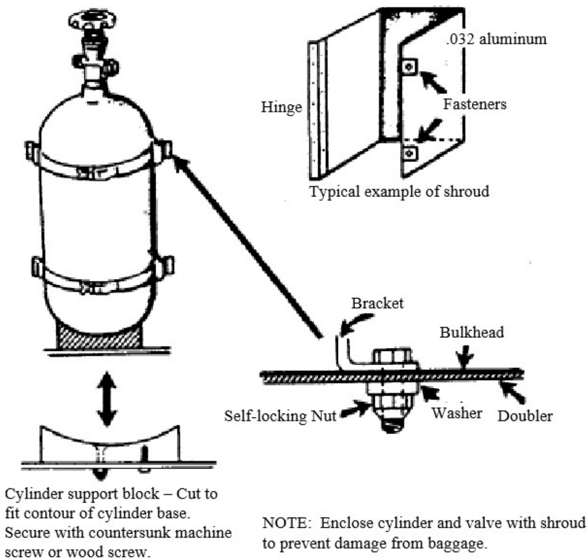
Figure 7-2. Typical Baggage Compartment Mounting
