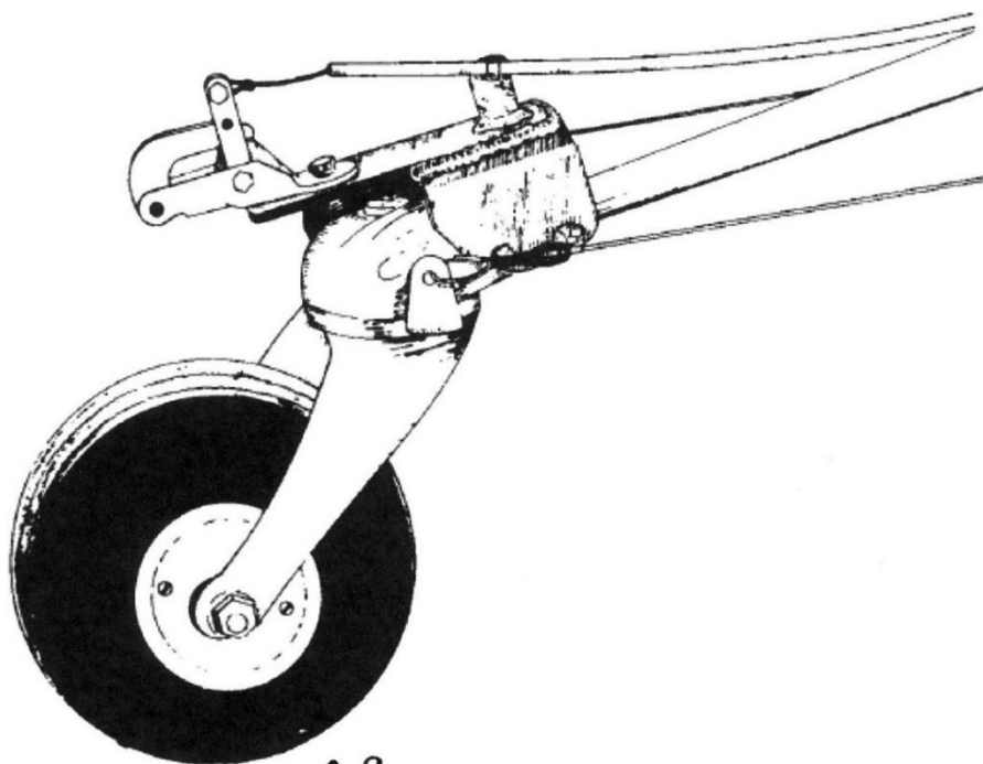
Figure 9-7. Conventional Gear Aircraft—Tubular Spring Type Tailwheel
